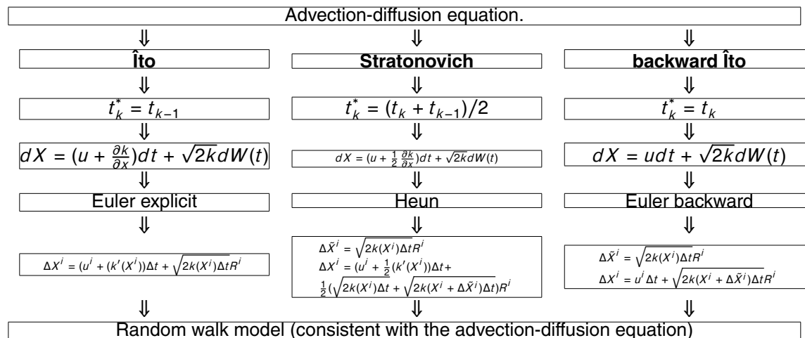
Fig. 1. Comparison between Itô, Stratonovich and backward Itô formulations.
