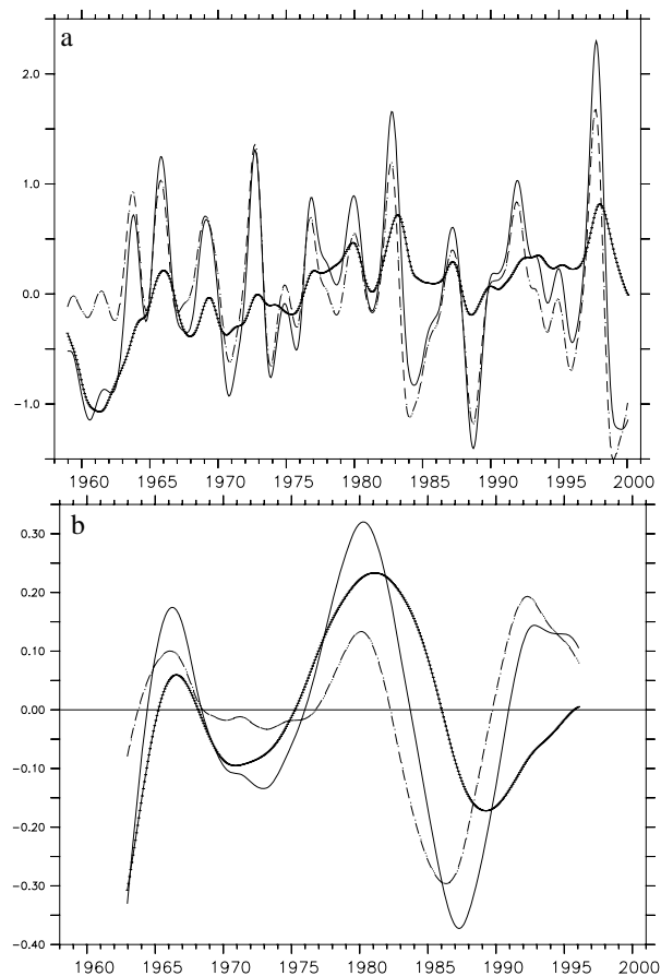
Fig. 8. T_{80} anomalies averaged over the Niño3 region for REF (solid line), EQ (dashed line) and NO EQ (dotted line); (a) interannually, (b) decadal smoothed.
