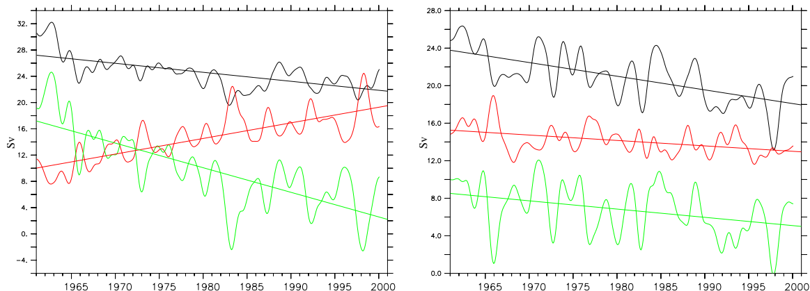
Fig. 11. Interannually smoothed net equatorward transport across (a) 6^{\circ} S to 10^{\circ} S and (b) 6^{\circ} N to 10^{\circ} N in the STC density range; total transport (black) separated into transport at the western boundary (red) and in the interior basin (green).
