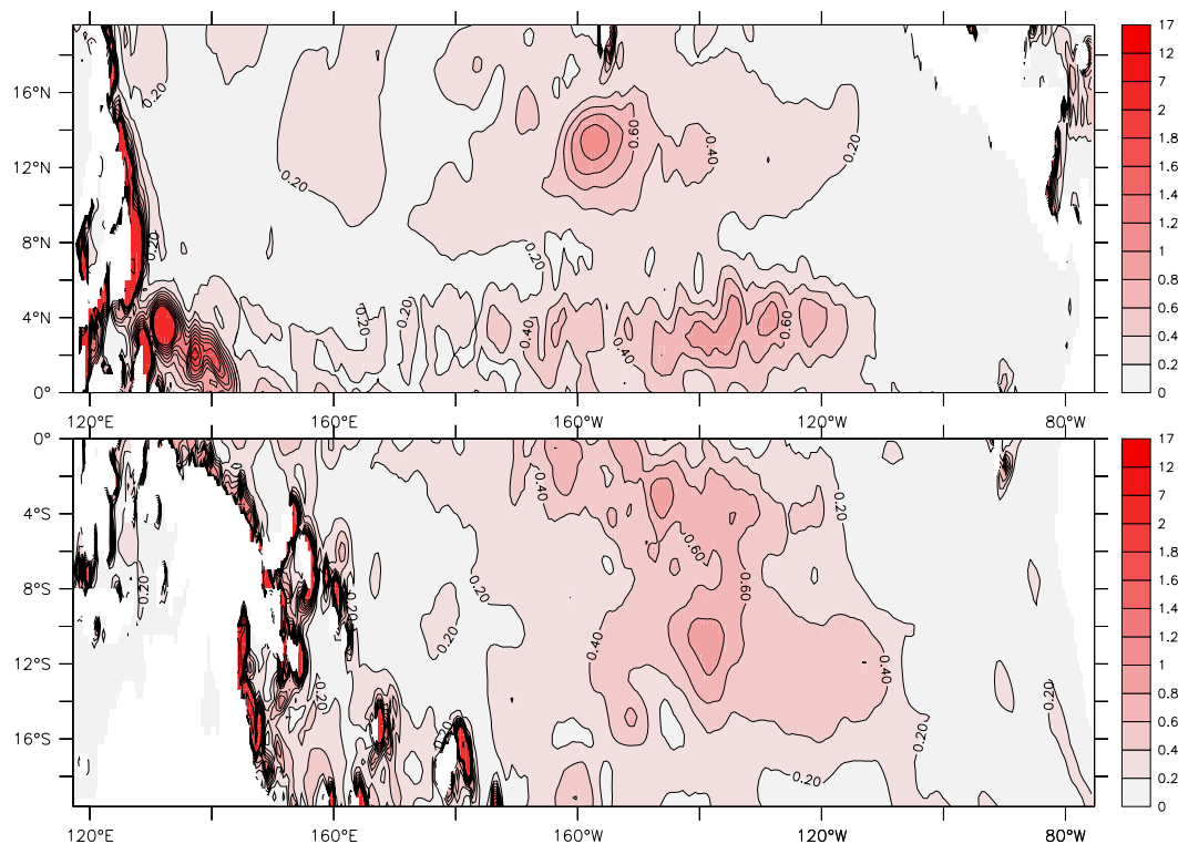
Fig. 10. Standard deviation of \nu\bar{T} , integrated across the density range of the equatorward layer ( \sigma=22.5 to 26.2 for the southern and \sigma=22.0 to 26.0 for the northern hemisphere) and decadal smoothed.
