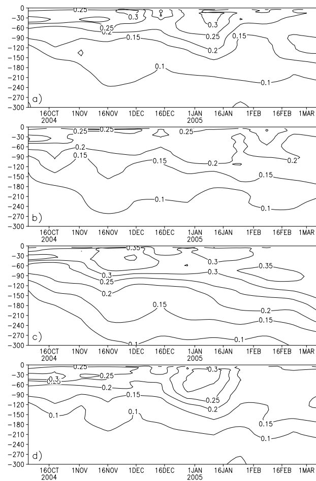
Fig. 5. Same as Fig. 4, but for salinity residuals (PSU) calculated with observations by ARGO floats.
