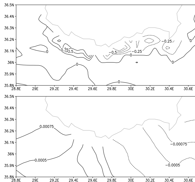
Fig. 6. The increment of the surface elevation (m) in the first model time step starting from the analysis on 1 October 2004. The figure shows a part of the coast where the un-initialised analysis produced particularly large oscillations of the surface elevation. The result for the un-initialised analysis is shown in the upper panel, and for the initialised analysis in the lower panel. The contour interval in the upper panel is 0.25 m and in the lower panel 0.00025 m.
