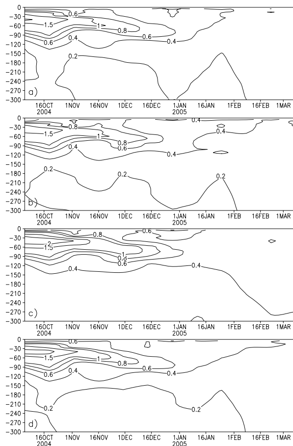
Fig. 4. The r.m.s. of temperature residuals in the first 500m of the water column ( ^{\circ}\text{C} ) calculated with observations by ARGO floats: (a) reference experiment, (b) weekly analyses, (c) analyses without the assimilation of ARGO floats and (d) analyses with unbalanced EOFs. The r.m.s. is averaged for a period of 14 days.
