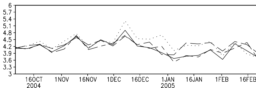
Fig. 3. The weekly r.m.s. of SLA residuals (m) in the period 1 October 2004–15 March 2005. The full line is for the reference experiment, the long dashed line for the experiment with the weekly analyses, the short-long dashed line for the experiment without the assimilation of observations by ARGO floats, and the dotted line for the experiment with un-balanced EOFs.
