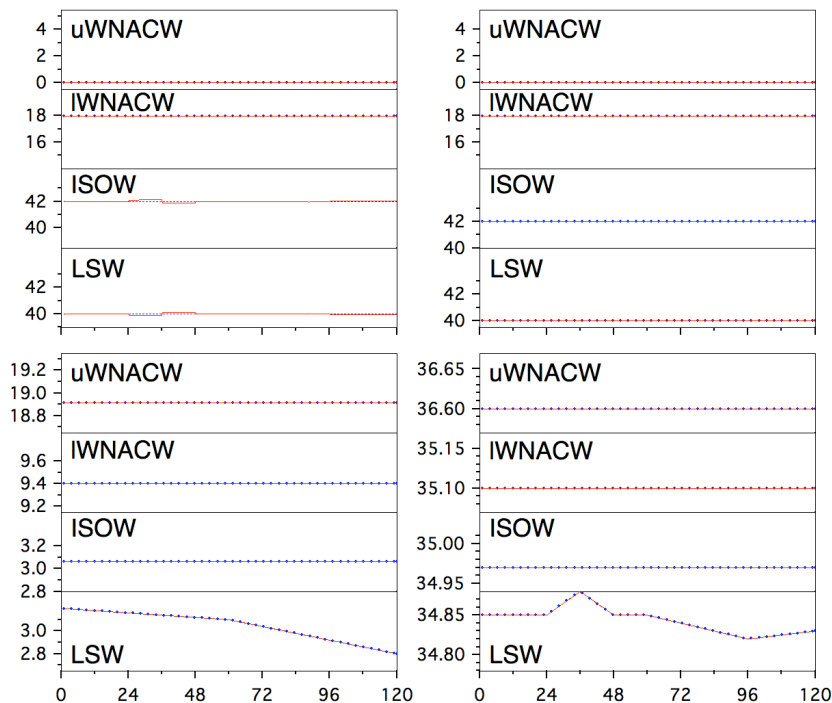
Fig. 5. Results of the analysis of data set 2 for the 1200 m depth level. Oxygen and nutrients were declared constants for all water masses, temperature and salinity for all water masses but LSW. Temperature and salinity of LSW were allowed to vary by up to 3% at every time step. Stages 1 and 2 went through 5 iterations at every time step. Relative water mass contributions (%) from the results of stage 1 (OMP analysis, top left) and after five iterations through stages 1 and 2 (TROMP analysis, top right); time development of potential temperature ( ^{\circ}\text{C} , bottom left) and salinity (bottom right). Red lines indicate calculated values. Dotted blue lines indicate the target values; where the difference between calculated and target values is not resolved in the graph, the target values are indicated by heavy blue dots. (At 1200 m the target value for uWNACW is zero). Axes are scaled to compare directly with Fig. 4.
