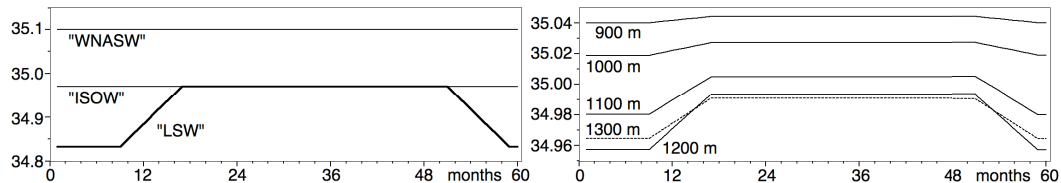
Fig. 1. Simulated data set 1 as a function of time. Left: Salinity of the source water types; right: salinity at five depth levels.
