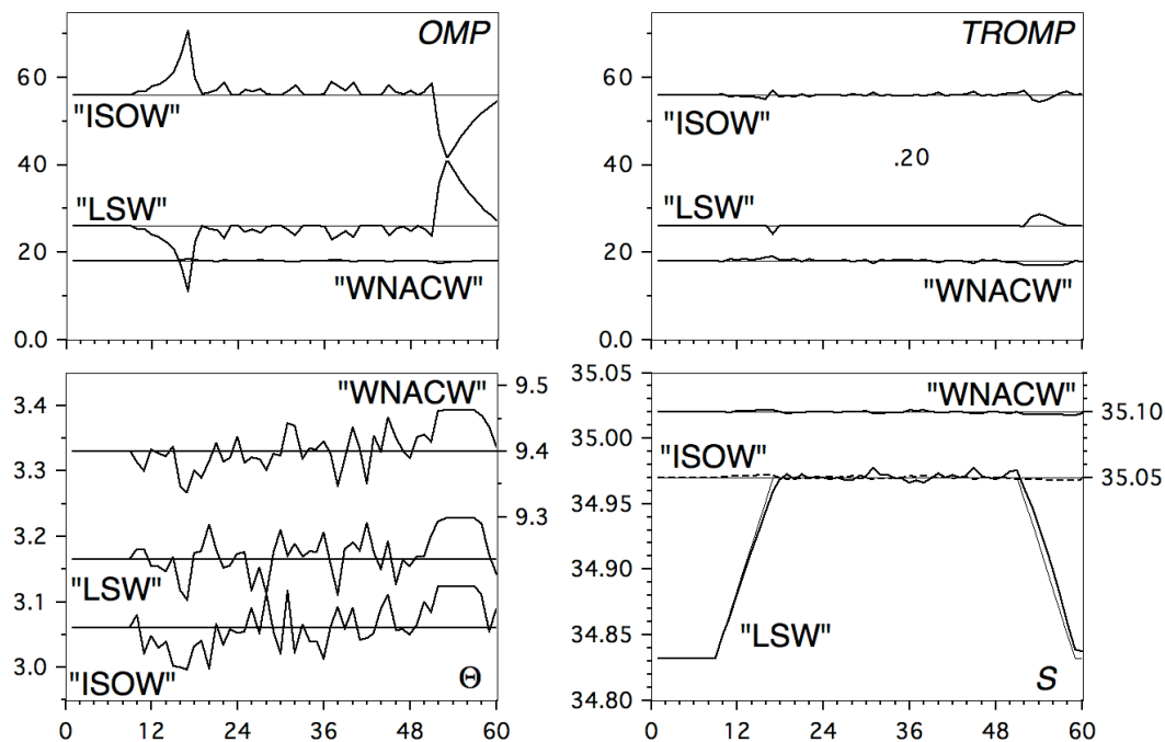
Fig. 3. Results of the analysis of data set 1 for the 1200 m depth level when LSW salinity is allowed to vary, all other source water properties are handled as variables with near-zero tolerance, and stages 1 and 2 go through 3 iterations at every time step. Relative water mass contributions (%) from the results of stage 1 (OMP analysis, top left) and after three iterations through stages 1 and 2 (TROMP analysis, top right); time development of potential temperature ( ^{\circ}\text{C} , bottom left) and salinity (bottom right). Thin lines indicate the target values.
