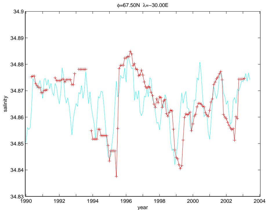
Fig. 9. The time series of DSO salinity (red) and the scaled difference of the mean sea level pressure (NCEP) between 67.5° N 30° W and Island (cyan).
