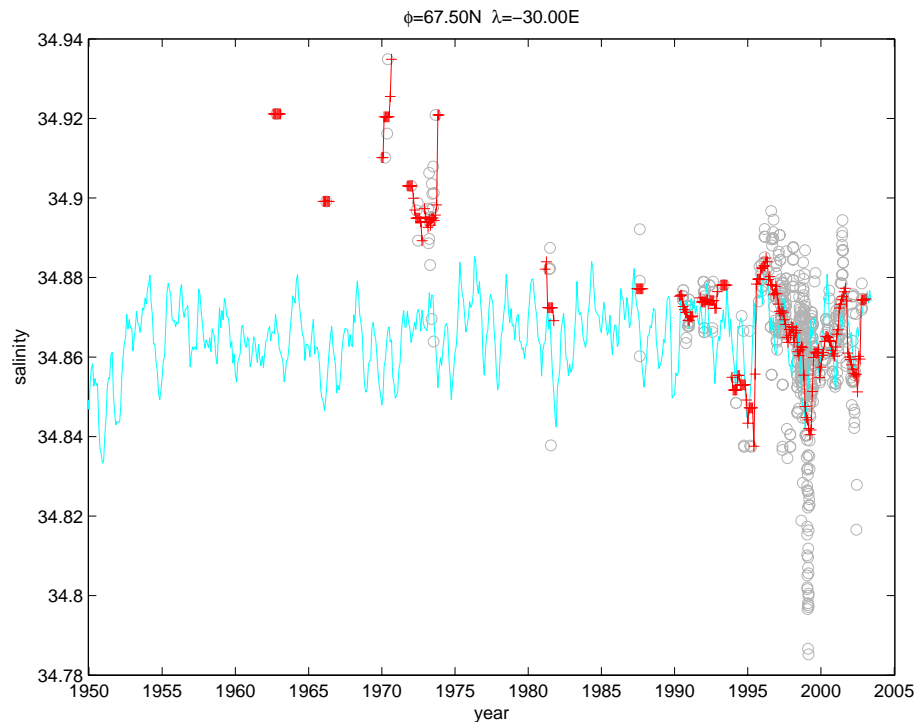
Fig. 10. Salinity of individual stations at \sigma_2=37.12 \text{ kg m}^{-3} (grey circles) and a running mean through this data giving the time series of the DSOW salinity (red) and the scaled difference of the mean sea level pressure between 67.5^\circ \text{ N} 30^\circ \text{ W} and Island (cyan) including also data before 1990.
