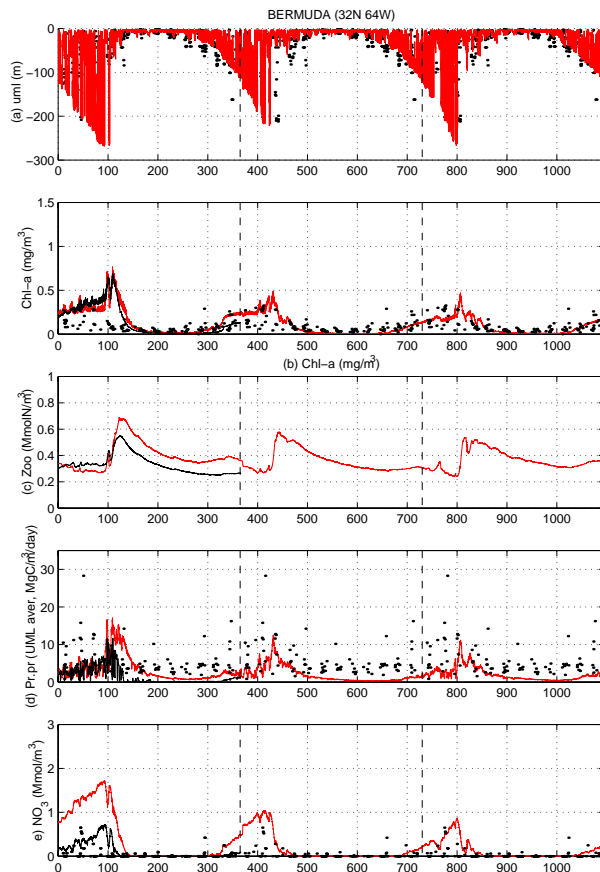
Fig. 2. Annual cycle of modelled (solid line) and observed (dots) ecosystem characteristics at BATS: (a) – UML depth (m), (b) – UML depth integrated Chl-a ( \text{mg Chl m}^{-3} ), (c) – surface zooplankton biomass ( \text{mmol N m}^{-3} ), (d) – UML averaged primary production ( \text{g C m}^{-3} \text{d}^{-1} ), (e) – surface nitrate concentration ( \text{mmol N m}^{-3} ). Results of the numerical experiment are shown for the first year as a thick line.
