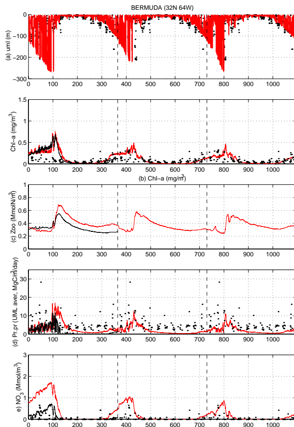
Fig. 2. Annual cycle of modelled (solid line) and observed (dots) ecosystem characteristics at BATS: (a) – UML depth (m), (b) – UML depth integrated Chl-a ( \text{mg Chl m}^{-3} ), (c) – surface zooplankton biomass ( \text{mmol N m}^{-3} ), (d) – UML averaged primary production ( \text{g C m}^{-3} \text{d}^{-1} ), (e) – surface nitrate concentration ( \text{mmol N m}^{-3} ). Results of the numerical experiment are shown for the first year as a thick line.
