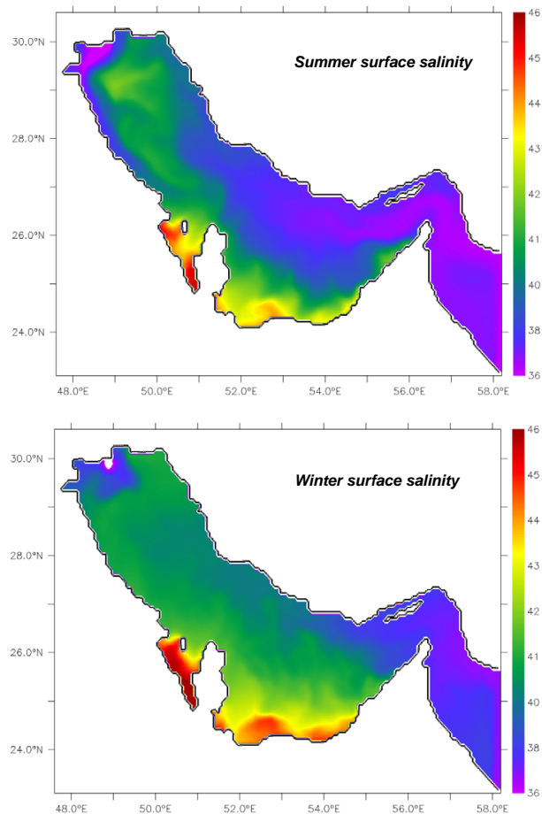
Fig. 12. Simulated surface salinities (psu) averaged over (top) summer months (June–August) and (bottom) winter months (December–February).
