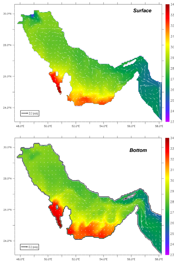
Fig. 10. Same as Fig. 8, but for winter months (December–February).
