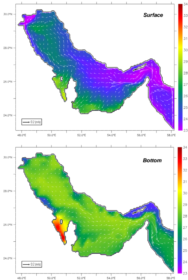
Fig. 8. Lateral distributions of surface and bottom flow vectors (arrows, \text{m s}^{-1} ) over density (colours, \sigma_t , \text{kg m}^{-3} ) averaged over summer months (June–August).
