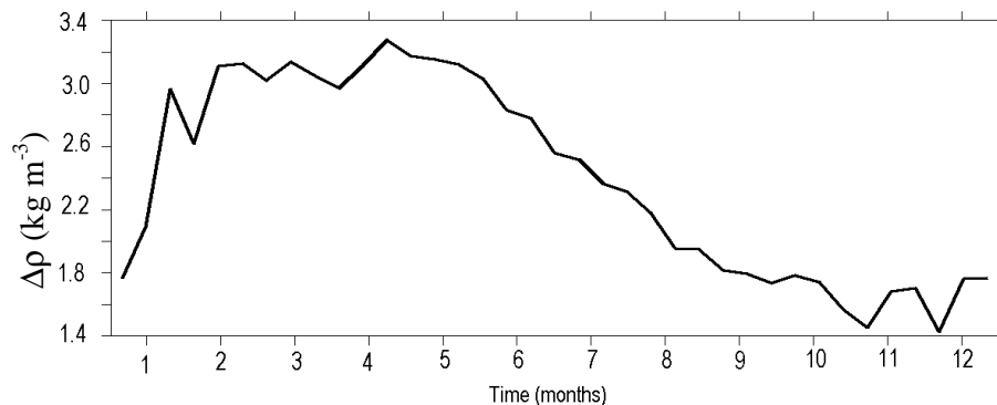
Fig. 6. Seasonal variations of the density difference at both sides of the Strait of Hormuz at a depth level of \sim 70 m.
