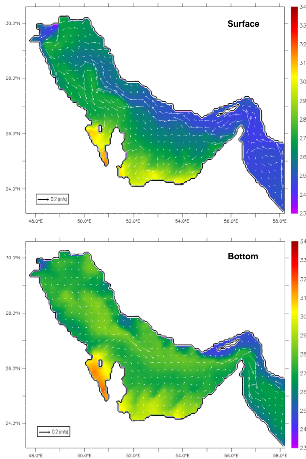
Fig. 9. Same as Fig. 8, but for autumn months (September–November).
