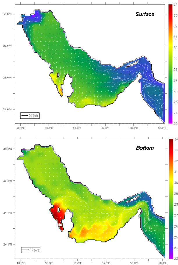
Fig. 11. Same as Fig. 8, but for spring months (March–May).
