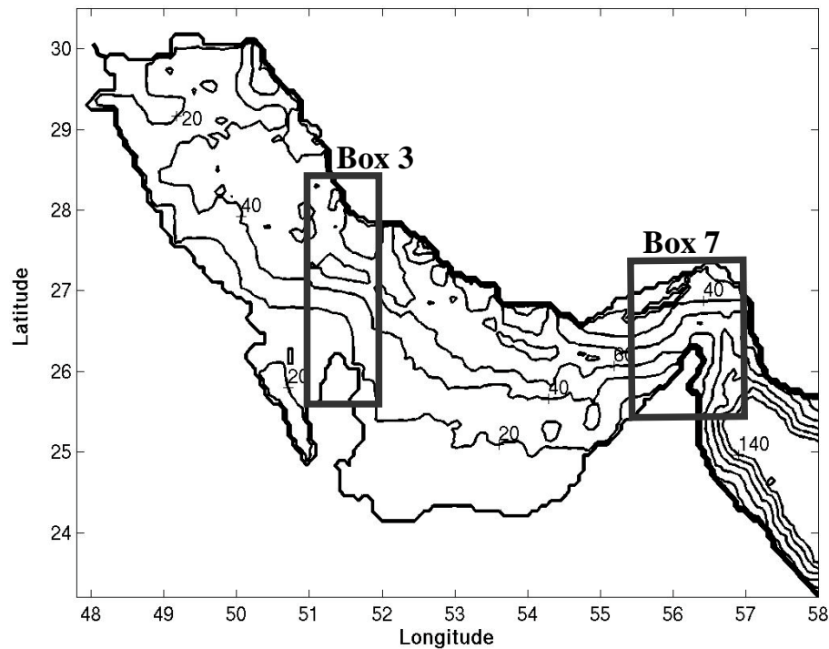
Fig. 4. Locations of boxes used for detailed analysis of hydrographic properties.
