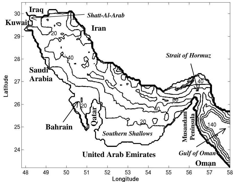
Fig. 1. Bathymetry (CI=20 m) used in this study.
