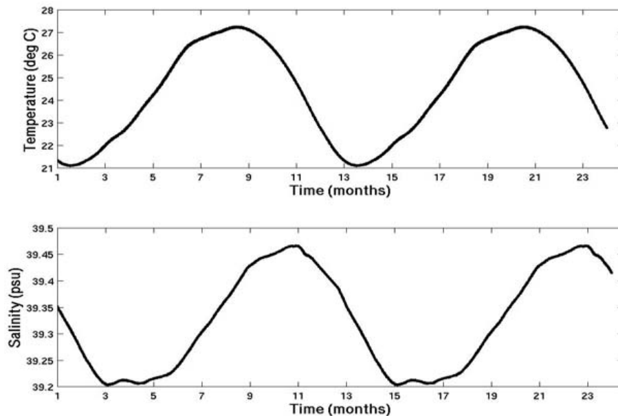
Fig. 2. Time series of domain-averaged temperature ( ^{\circ}\text{C} , top panel) and salinity (psu, bottom panel) for the last two years of the simulation.
