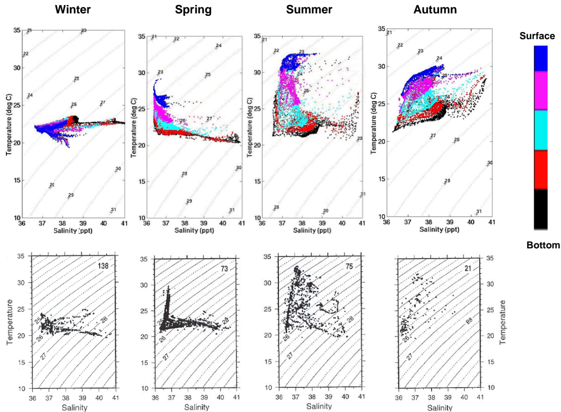
Fig. 5. Temperature-salinity-season diagrams for the Strait of Hormuz. (top) Model predictions. Colours indicate sigma levels. (bottom) Field observations, taken from Alessi et al. (1999).
