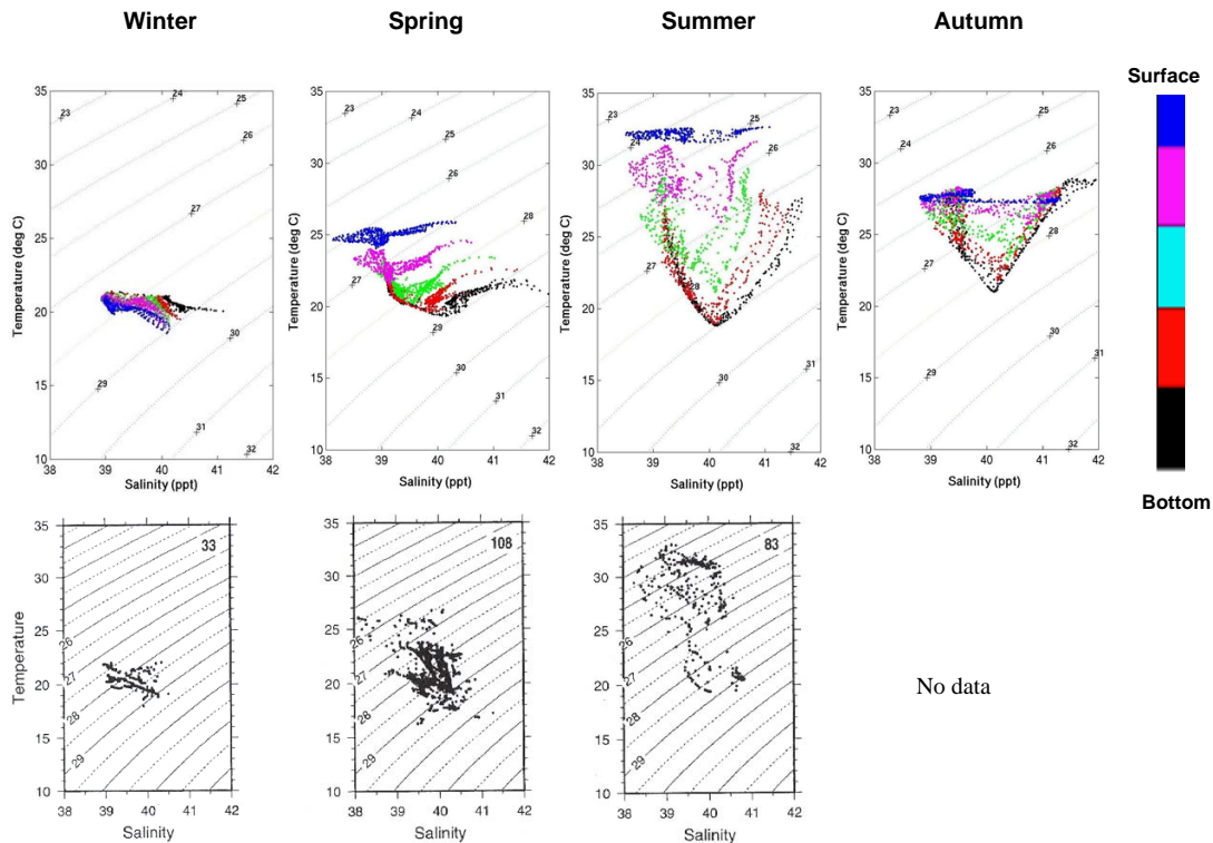
Fig. 7. Same as Fig. 5, but for central regions (Box 3) of the Persian Gulf.
