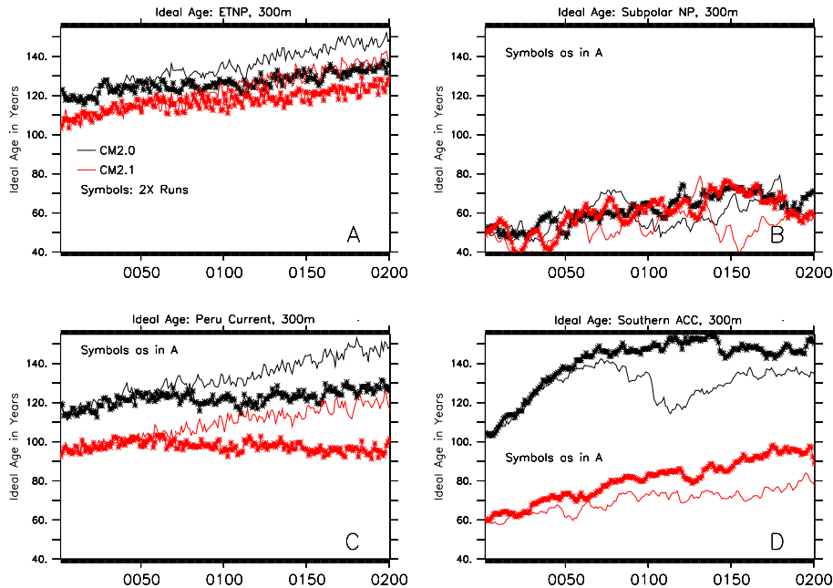
Fig. 5. Time series of the ideal age at 300 m in the CM2 series. Black lines are for CM2.0, red for CM2.1. Lines with symbols are the doubled \text{CO}_2 run. (A) Eastern Tropical North Pacific. Note that the ages under global warming begin to diverge about year 50. (B) Subpolar North Pacific. Note substantial decadal variability of same order of magnitude as climate change. (C) Peru Current. Here the difference between the ages cannot be attributed to spinup alone, as year 80 of the control CM2.1 is still substantially younger than CM2.0. (D) Southern Ocean. The same difference in age is attributable to a difference in ventilation forced by the higher Southern Ocean winds.
