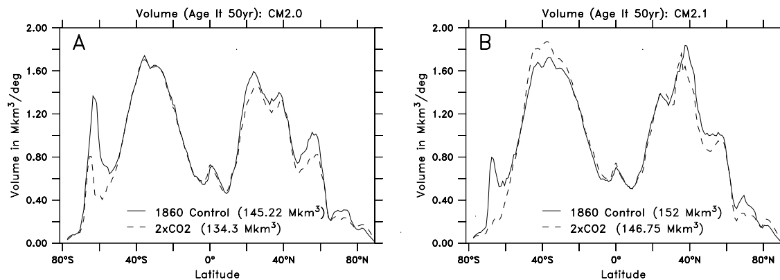
Fig. 4. Volume of “young” water (with an ideal age less than 50 years) in the CM2 series. Solid lines are the 1860 control, dashed lines the doubled carbon dioxide run. (a) CM2.0. (b) CM2.1.
