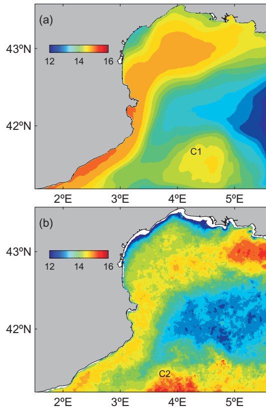
Fig. 7. (a) Time-averaged model surface temperature (°C). The anticyclonic eddy is indicated with C1. (b) Monthly-averaged satellite (AVHRR) SST (°C) for December 2005. CThe anticyclonic eddy is indicated with C2.
