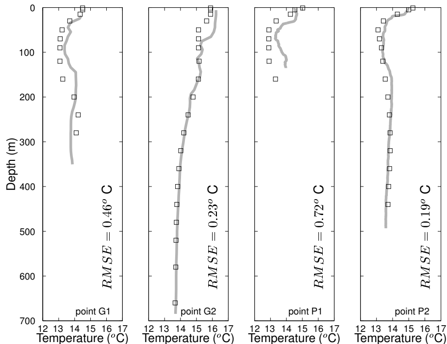
Fig. 6. Measured in-situ temperature profiles (thick grey line) and interpolated model output (black squares) obtained from Med-Argo gliders (G1, G2) and VOS-XBT (P1, P2). The root mean square error (RMSE) is added for each plot. For spatial coordinates see Fig. 1.
