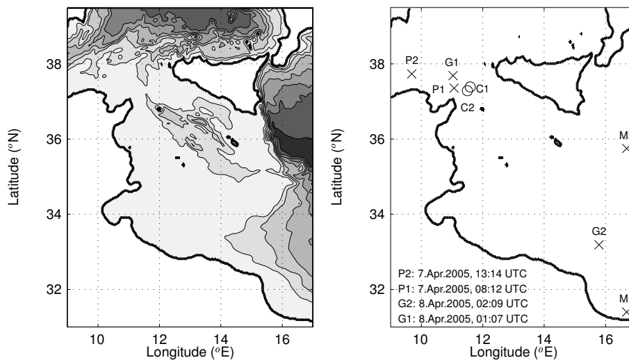
Fig. 1. The SCRM domain with bathymetry in grey contours from light (shallow) to dark (deep), contour interval 500m. The thick black line represents the coast line. Locations of in-situ measurements with XBT profilers are indicated with P1 and P2, Med-Argo gliders with G1 and G2, and with chained current meters with C1 and C2. Two additional points (M1,M2) indicate the location of model output points used for frequency analysis.
