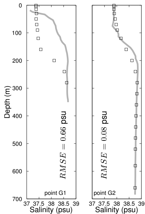
Fig. 7. Measured in-situ salinity profiles (thick grey line) and interpolated model output (black squares) obtained from Med-Argo gliders (G1, G2). For spatial coordinates see Fig. 1.
