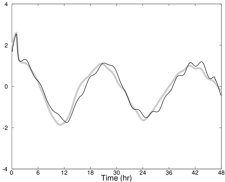
Fig. 5. Time series of a detrended and normalized u component of velocity optimized with VIFOP (thick grey line) and non-optimized (thin black line) at M2 (Fig. 1).
