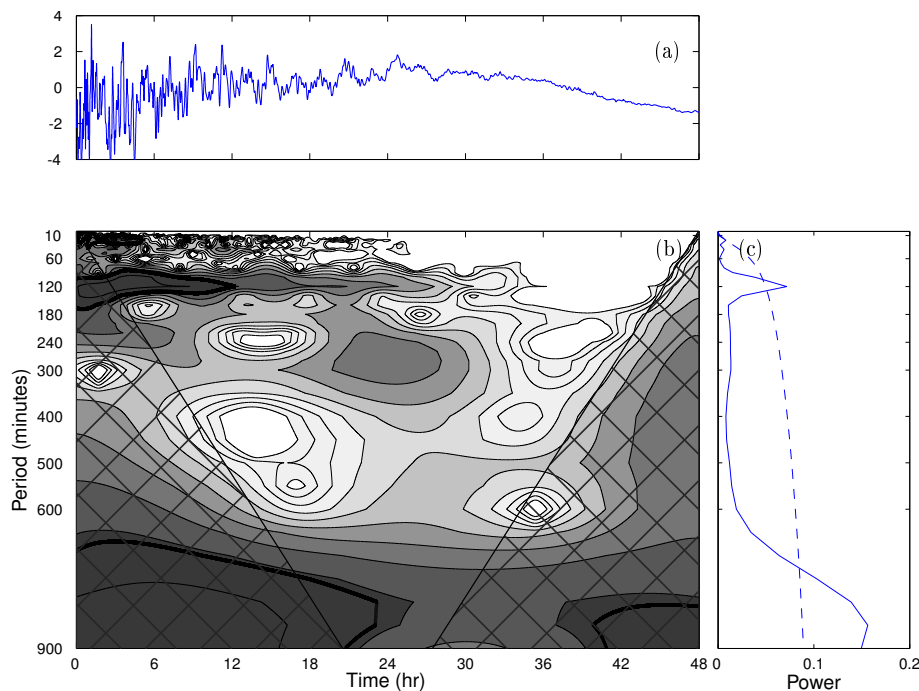
Fig. 3. (a) Time series of a detrended and normalized free surface elevation at i=248 , j=153 ( \varphi=35.75^\circ N, \lambda=16.7^\circ E). (b) Wavelet power spectrum of the same time series. The contour interval values for normalized variance are from light to dark in range [1, 2, \dots, 10] . The thick black line indicated the 95% confidence level for a red noise background, the hashed region represents the cone of influence. (c) The global power spectrum, with the 95% confidence level (dashed line). See text for a more detailed explanation.
