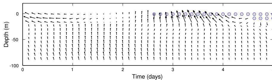
Fig. 11. Same as Fig. 10c, except for the point C1. Maximum velocity was approximately 0.9 \text{ ms}^{-1} . Circles denote missing values.
