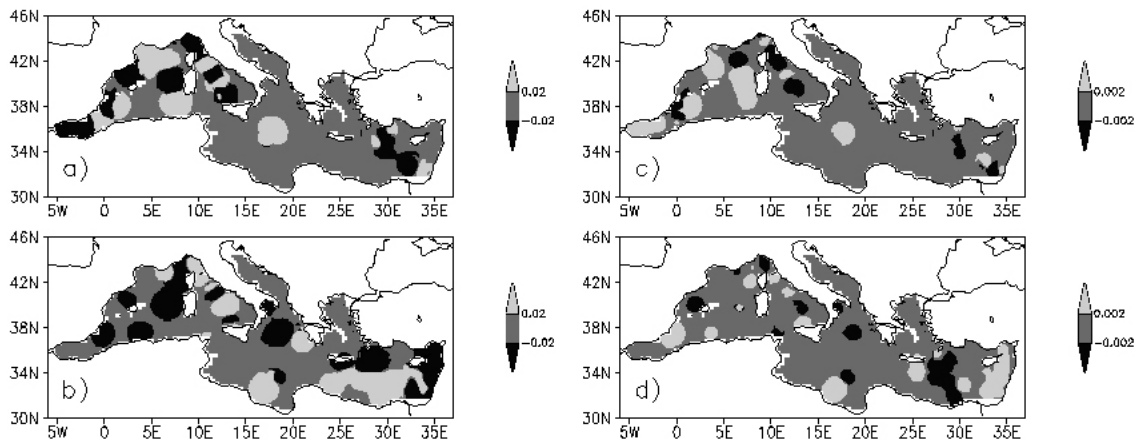
Fig. 14. Maps of corrections at 5 m depth after the first assimilation cycle (day 7) with sampling strategy VtARGO. Left panels: temperature (6°C) in summer (a) and winter (b). Right panels: salinity (psu) in summer (c) and winter (d).
