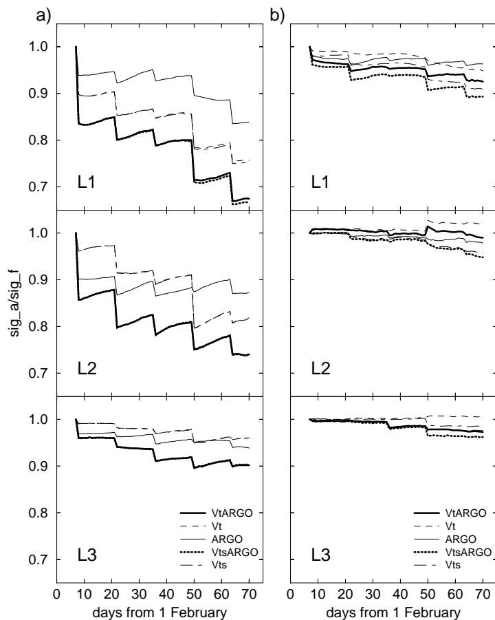
Fig. 13. Time series of temperature (a) and salinity (b) relative errors for the East Mediterranean in the winter OSSEs for real sampling strategies. L1 indicates the surface layer, L2 the intermediate layer and L3 the deep layer.
