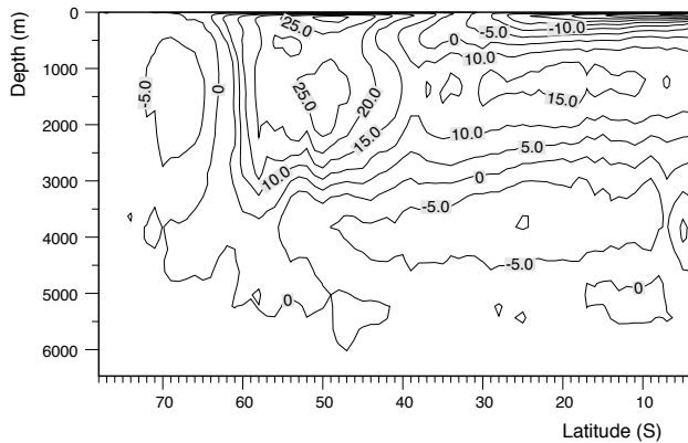
Fig. 3. Meridional overturning streamfunction for the control run at day 3692, after two days of the analysis period. Contour values are in Sverdrups ( 1 \text{ Sv} = 10^6 \text{ m}^3 \text{ s}^{-1} ).
