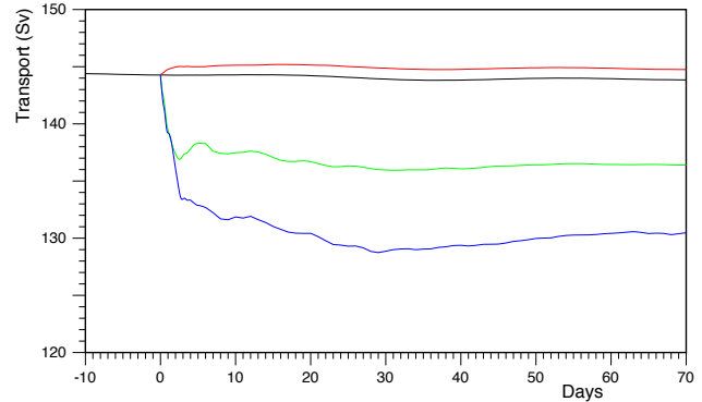
Fig. 2. Drake Passage transport during the analysis period. The lines are: Black – the control run; Red – perturbation run, zonal wind stress increased by 0.01 \text{ Nm}^{-2} at the latitudes of Drake Passage; Green – zonal wind stress set to zero at the same latitudes; Blue – wind stress set to zero everywhere. Days measured relative to day 3690 at the start of the analysis period.
