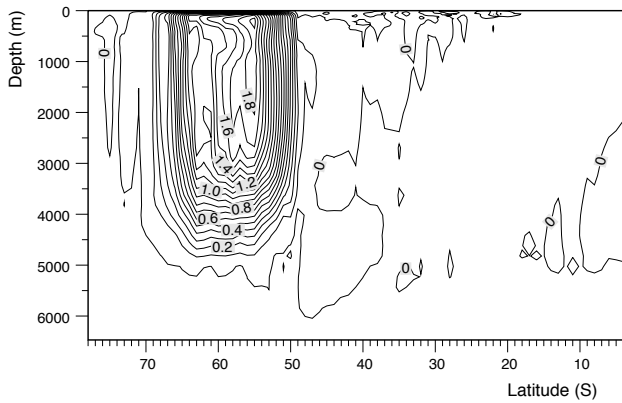
Fig. 4. Difference in the meridional overturning streamfunction between the perturbation run (Run 2 – an additional 0.01 \text{ Nm}^{-2} wind stress at the latitudes of Drake Passage) and the control run after two days.
