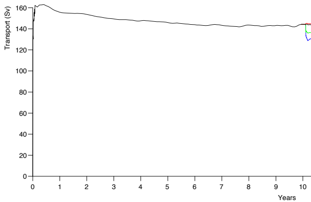
Fig. 1. Drake Passage transports during the spin up and test periods. The lines are: Black – the control run; Red – perturbation run, zonal wind stress increased by 0.01 \text{ Nm}^{-2} at the latitudes of Drake Passage; Green – zonal wind stress set to zero at the same latitudes; Blue – wind stress set to zero everywhere. Transport in Sverdrups ( 1 \text{ Sv} = 10^6 \text{ m}^3 \text{ s}^{-1} ).
