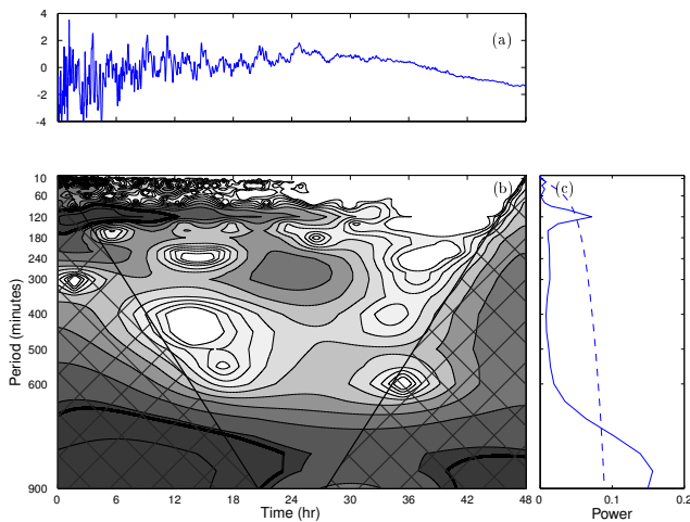
Fig. 3. (a) Time series of a detrended and normalized free surface elevation at i=248, j=153 ( \phi=35.75^\circ N, \lambda=16.7^\circ E). (b) Wavelet power spectrum of the same time series. The contour interval values for normalized variance are from light to dark in range [1, 2, , 10]. The thick black line indicated the 95% confidence level for a red noise background, the hashed region represents the cone of influence. (c) The global power spectrum, with the 95% confidence level (dashed line). See text for a more detailed explanation.
