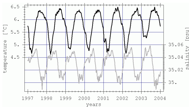
Fig. 13. Low-pass filtered (cut-off frequency: (30 \text{ days})^{-1} ) simulated temperature (upper black curve) and salinity (lower grey curve) at section 3b (mean between surface and 800 m depth) south of Denmark Strait.
