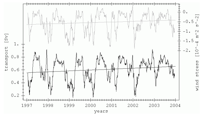
Fig. 10. 31 day moving averages of the southward wind stress component (NCEP) (divided by the water density of 1030 kg m -3 ) at 67°40' N, 22°32' W (upper curve) and simulated volume flux of the NIIC normal to section 7 (lower curve). Trends 1997–2003 are: 3.2 \times 10^{-6} \text{ m}^2 \text{ s}^{-2} per year for the wind stress, and 0.014 Sv per year for the volume flux.
