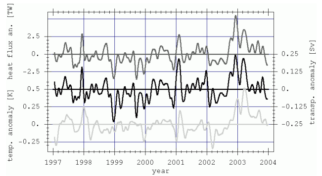
Fig. 11. Low-pass filtered (cut-off frequency: (30 days) -1 ) anomalies relating to the seasonal signals shown in Fig. 9. The uppermost, dark-grey curve shows simulated NIIC heat flux anomalies at section 7. The black curve in the middle shows the NIIC's volume flux anomalies normal to section 7. The light-grey curve below shows the spatially averaged water temperature anomaly over the North Icelandic shelf (area between sections 7 and 12 with water depth below 300 m).
