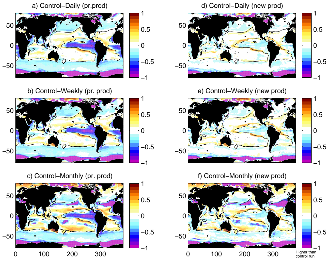
Fig. 7. Deviation of the mean annual primary production in the control run (see Fig. 5 for additional explanation) from the daily forcing run (a), weekly forcing run (b), monthly forcing run (c); deviation of the mean annual new production in the control run from the daily forcing run (d), weekly forcing run (e), monthly forcing run (f). Black dots show the locations of the five time series stations discussed in the text and shown on Figs. 2 and 10.
