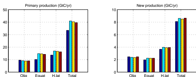
Fig. 8. Mean annual primary (a) and new (b) production ( \text{GtC yr}^{-1} ) integrated over the equatorial, oligotrophic and high latitude areas (see text) and the global ocean for the 6 h (dark blue), daily (light blue), weekly (yellow) and monthly (red) forcing runs.
