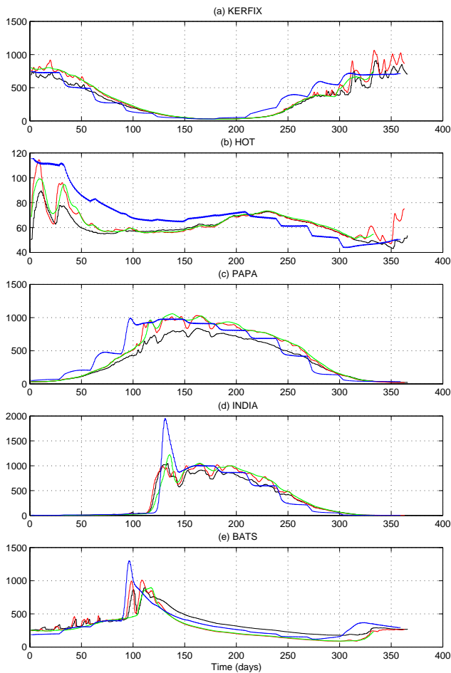
Fig. 10. Photic zone integrated primary production ( \text{mgC m}^{-2} \text{d}^{-1} ) for the year 1992 at KERFIX (a), HOT (b), Papa (c), India (d), BATS (e) in the control run (black), daily (red), weekly (green) and monthly (blue) forcing runs.
