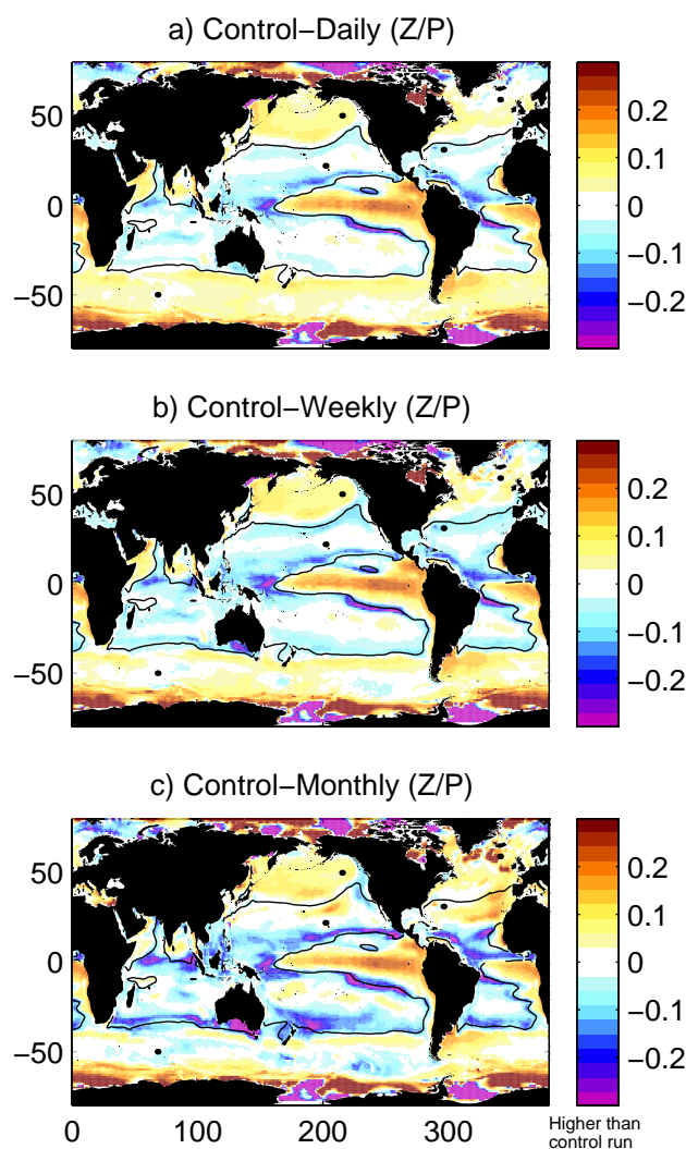
Fig. 9. Deviation of the surface phyto- to zooplankton ratio in the control run (see Fig. 5 for additional explanation) from the daily forcing run (a), weekly forcing run (b), monthly forcing run (c). Black dots show the locations of the five time series stations discussed in the text and shown on Figs. 2 and 10.
