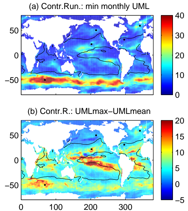
Fig. 3. (a) The monthly-averaged UML depth from the control run for the month when it is at its minimum, in m. (b) Difference (in m) between the minimum monthly averaged daily maximum (night-time) UML depth and the minimum monthly-averaged UML depth. Black dots show the locations of the five time series stations discussed in the text and shown on Figs. 2 and 10. Black line represents a mean annual nitrate concentration of 1 \text{ mmol m}^{-3} also shown in Figs. 4, 7, 9, and chosen as a means of defining the boundaries between different regions described in the text.
