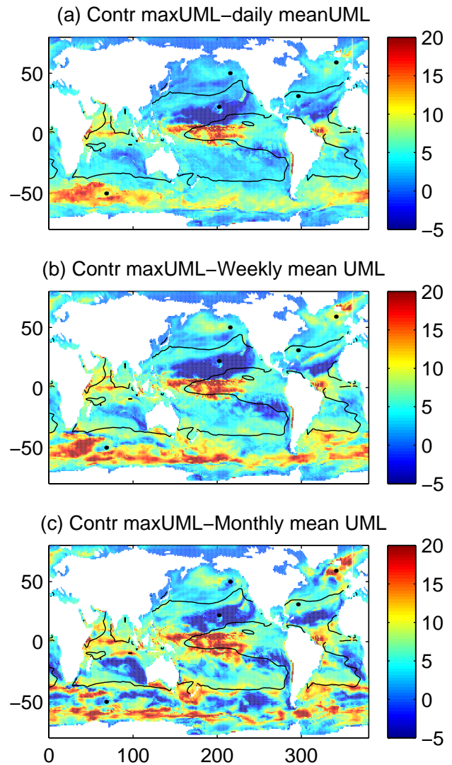
Fig. 4. Difference (in m) between the minimum monthly averaged daily maximum (night-time) UML depth in the control run and the minimum monthly-averaged UML depth in the runs driven by daily averaged (a), weekly averaged (b) and monthly averaged (c) forcing.
