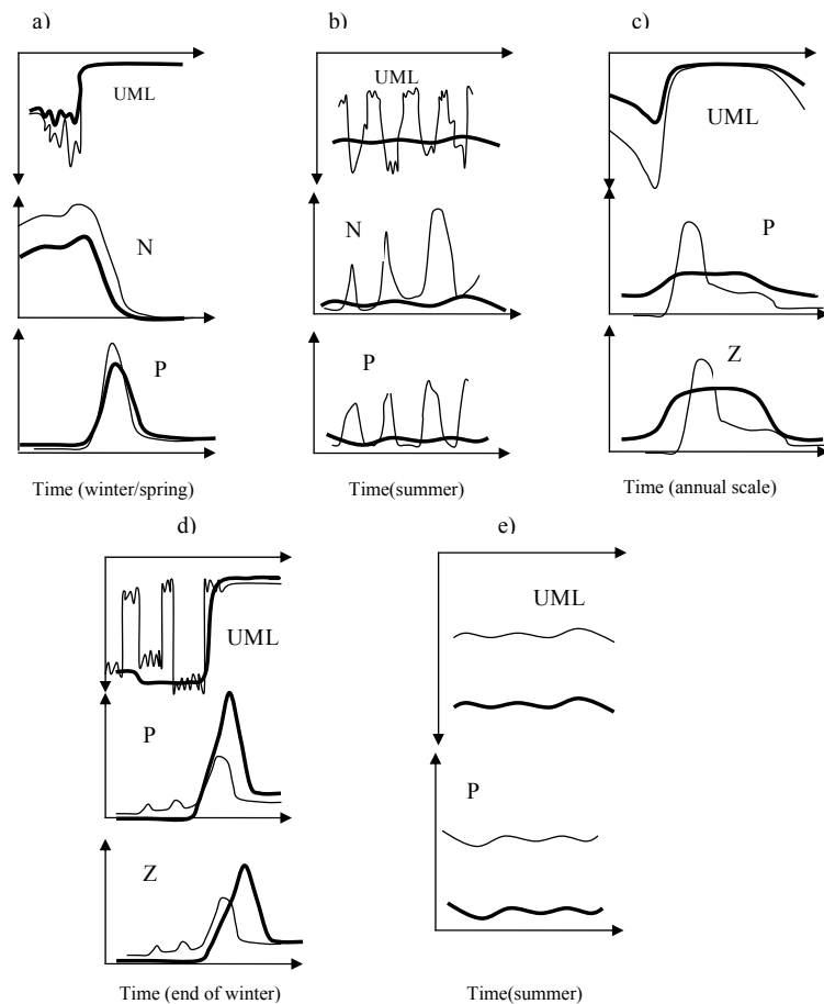
Fig. 1. Schematic representation of the main UML control mechanisms over ecosystem dynamics: (a) Impact of depth of winter mixing (the major factor determining nutrient supply to the UML). Thick line describes a shallower (compared with the thin line) winter convection leading to lower nitrate concentration in the UML at the beginning of the spring, and a lower phytoplankton bloom terminated earlier by nutrient limitation. (b) Impact of short-term storm-induced summer deepening of the UML (enhances nutrient supply into the photic zone and primary production if it is nutrient-limited as opposed to light-limited). Thin line describes frequent deepening of the UML as opposed to the stable depth (thick line) leading to the pulses of nutrients entrained from below the UML leading to an increase in phytoplankton biomass. (c) Impact of average winter mixing depth (influences the extent to which zooplankton can survive through the winter and hence exert grazing pressure on the spring phytoplankton bloom). The thin line describes a deeper (compared with the thick line) winter convection when primary production is low during the winter because of strong light limitation, leading to low zooplankton biomass which does not then put a significant grazing pressure on the spring phytoplankton bloom. In the case described by the thin line, zooplankton grazing suppresses the spring bloom. (d) Impact of short-term re-stratification of the UML during late winter and spring due to extremely calm weather followed by the return of deep mixing (such periods reduce light limitation and increase the level of coupling between phytoplankton and their grazers and change the dynamics of the spring bloom). Thin line describes a convective regime with a frequent near-surface re-stratification allowing significant production to occur, followed by the growth of zooplankton. At the moment of the spring bloom zooplankton population is then large enough to exert a significant grazing pressure on the phytoplankton. In the case of stable deep convection (thick line), the zooplankton population at the moment of the bloom is low and the first stage of the bloom develops without grazing pressure. (e) Impact of average summer mixed layer depth (determines light limitation of phytoplankton growth over the season). The thick line describes deeper (compared with the thin line) UML depth leading to higher light limitation of primary production and lower phytoplankton biomass.
