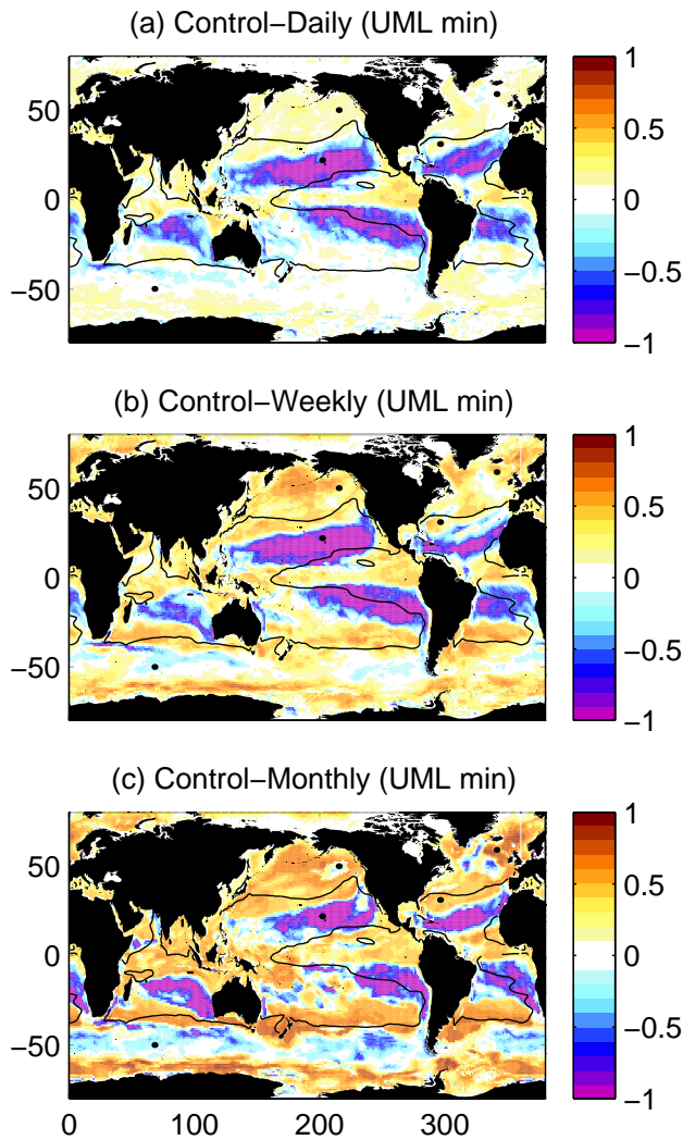
Fig. 5. Differences at each point between the minimum monthly UML depth in the control run and in the runs driven by daily-averaged (a), weekly-averaged (b) and monthly-averaged (c) forcing, divided by the minimum monthly UML depth in the control run at that point. Differences in the following figures (except Fig. 6b) are also calculated in this way as \frac{X_{\text{control}} - X_{\text{experiment}}}{X_{\text{control}}} . Negative values highlight areas where averaging of the forcing fields leads predicted summer-time UMLs being deeper than in the 6 h run. These areas include equatorward regions of the subtropical gyres, with station HOT being situated in one such area. Regions showing positive values which include the poleward parts of the subtropical gyres as well as moderate and high latitude areas of the Northern hemisphere, show shallower predicted UMLs when the forcing is averaged. Black dots show the locations of the five time series stations discussed in the text and shown on Figs. 2 and 10.
