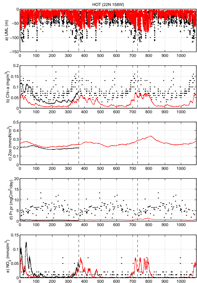
Fig. 3. Annual cycle of modelled (solid line) and observed (dots) ecosystem characteristics at HOT: (a) – UML depth (m), (b) – surface Chl-a ( \text{mg Chl m}^{-3} ), (c) – surface zooplankton biomass ( \text{mmol N m}^{-3} ), (d) – UML integrated primary production ( \text{mg C m}^{-2} \text{d}^{-1} ), (e) – surface nitrate concentration ( \text{mmol N m}^{-3} ). Results of the grazing experiment are shown for the first year as a black line.
