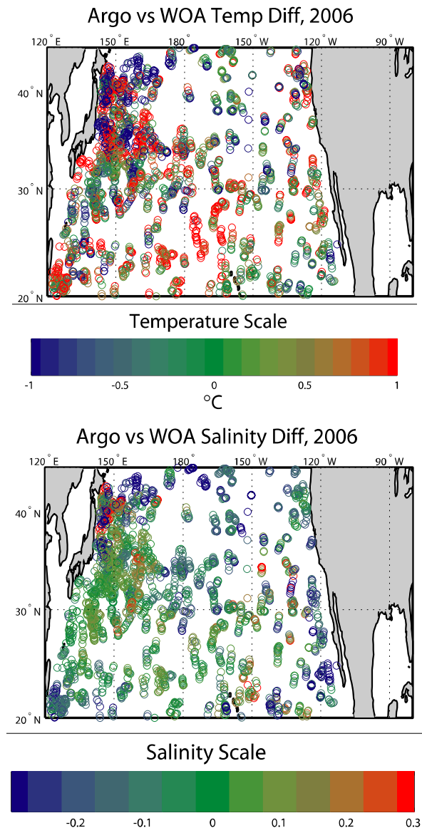
Fig. 6. Difference between Argo float and local WOA01 values at 10 m depth. (a) 2006 Temperature. (b) 2006 Salinity. At bottom are color scales for (a–b).
