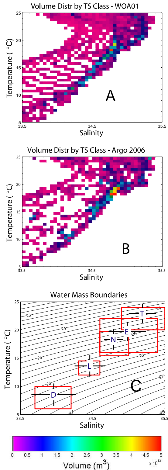
Fig. 2. (a) and (b) Distribution of water volume in the mixed layer by temperature and salinity class. Temperature and salinity are summed over ranges of 0.5^\circ\text{C} and 0.05 respectively. (a) WOA01. (b) Argo 2006. (c) T-S diagram showing the boundaries of the water masses discussed in the text and shown in Table 1. Also shown are medians and standard deviations of T-S properties for Argo 2005, cases 2 and 3 in the text. The median is indicated by letters: T – NPTW; E – ESTMW; N – NPSTMW; L – LCMW; D – DCMW. Standard deviations are indicated by bars. Potential density contours are shown in panel (c). (d) Color scale for panels (a) and (b).
