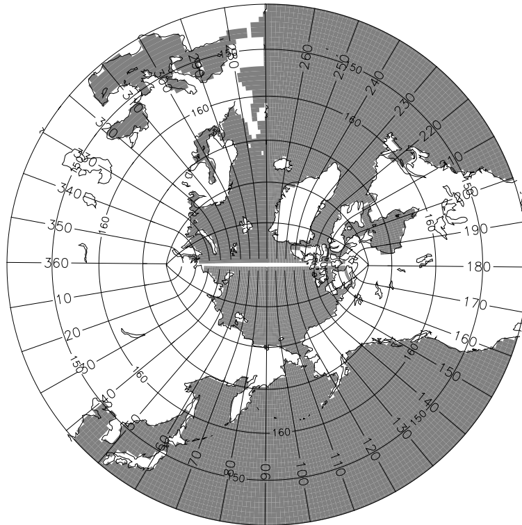
Fig. 1. Illustration of the bipolar Arctic as prescribed by Murray (1996) (see his Fig. 7) and realized in OM3. The transition from the bipolar Arctic to the spherical grid occurs at 65^\circ N. We denote horizontal grid cells by (i, j) indices. As in the spherical coordinate region of the grid, lines of constant i -index move in a generalized eastward direction within the bipolar region. They start from the bipolar south pole at i=0 , which is identified with i=ni , where ni is the number of points along a latitude circle and ni=360 in OM3. The bipolar north pole is at i=ni/2 , which necessitates that ni be an even number. Both poles are centered at a velocity point on the B-grid used in MOM4.0. Lines of constant j move in a generalized northward direction. The bipolar prime-meridian is situated along the j -line with j=nj , where nj=200 in OM3. This line defines the bipolar fold that bisects the tracer grid. Care must be exercised when mapping fields across this fold. As noted by Griffies et al. (2004), maintaining the exact identity of fields computed redundantly along the fold is essential for model stability. Note that the cut across the bipolar fold is a limitation of the graphics package, and does not represent a land-sea boundary in the model domain.
