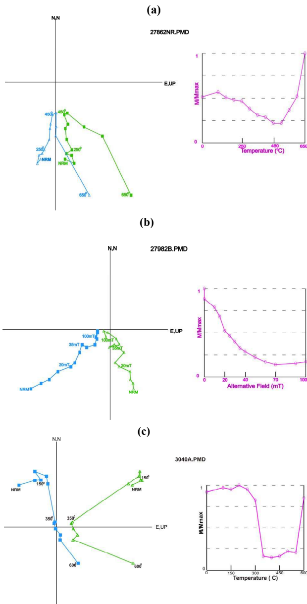
Fig. 3. Zijderveld diagrams and normalized magnetic intensity curves with stepwise AF thermal (a) and AF (b) demagnetization for representative samples. (c) Zijderveld diagram showing the viscous component (NRM to 150°C). Open triangles: projection onto the vertical plan, Black squares: projection onto the horizontal plan.
