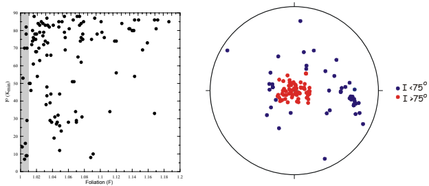
Fig. 9. Inclination values versus foliation (left) and equal area projections (lower hemisphere) of the direction of K_{\min} axis of anisotropy of the samples (right), in specimen coordinates.
