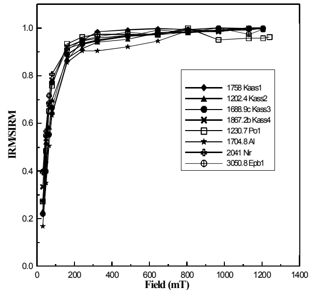
Fig. 4. IRM acquisition curves for representative samples.
