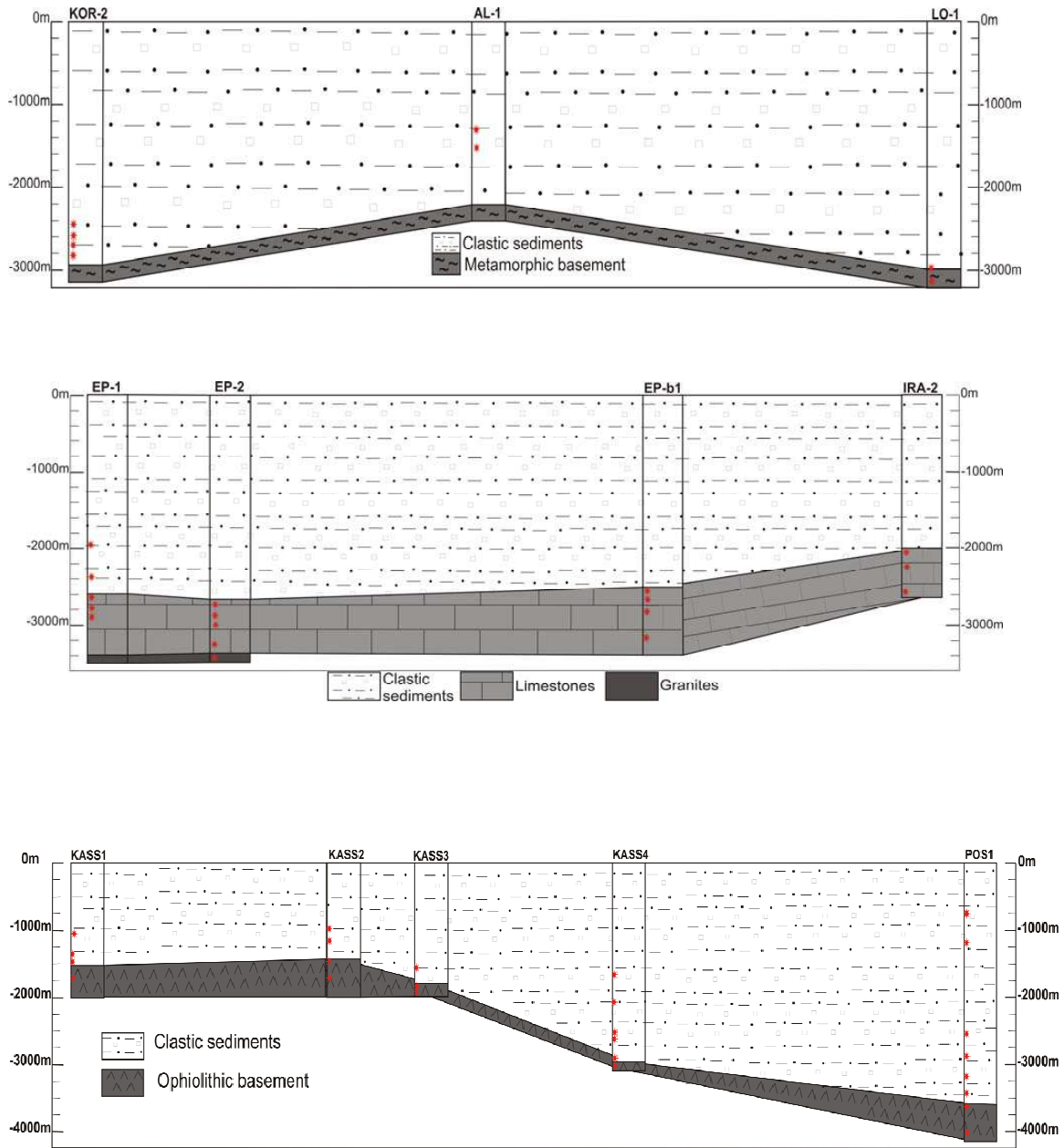
Fig. 2. Lithostratigraphy of all studied cores. Red dots show the depths where drill cores were taken.
