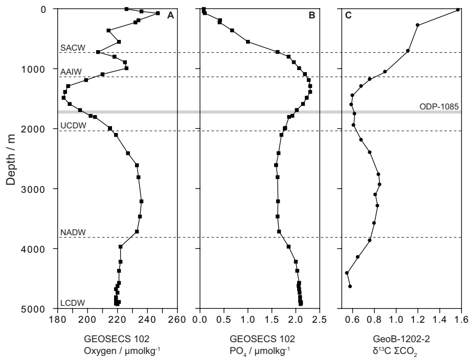
Fig. 2. Dissolved oxygen, phosphate, and \delta^{13}\text{C} \Sigma\text{CO}_2 profiles from GEOSECS 102 and GeoB-1202 (Bickert and Wefer, 1999), with delineations of the main deep water masses in the Cape Basin. The depth of studied core ODP-1085 is marked with a shaded horizontal band.
