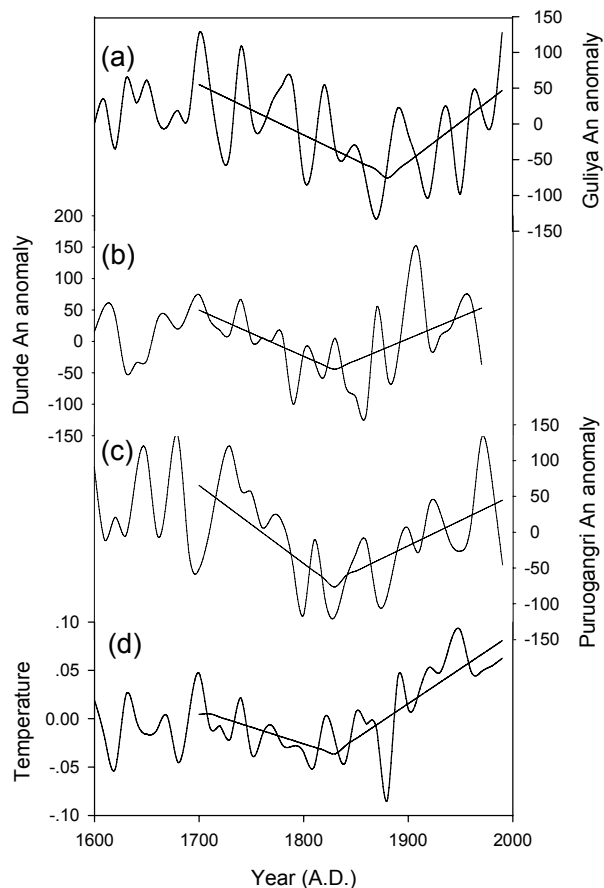
Fig. 4. Decadal changes of precipitation based on glacial accumulation reconstructed from Guliya ice core (a), Dunde ice core (b), and Puruogangri ice core (c). The decadal temperature reconstructed by the composition of \delta^{18}\text{O} from Puruogangri, Guliya and Dunde ice core (d). The thick lines are linear trends of precipitation and temperature reconstructions.
