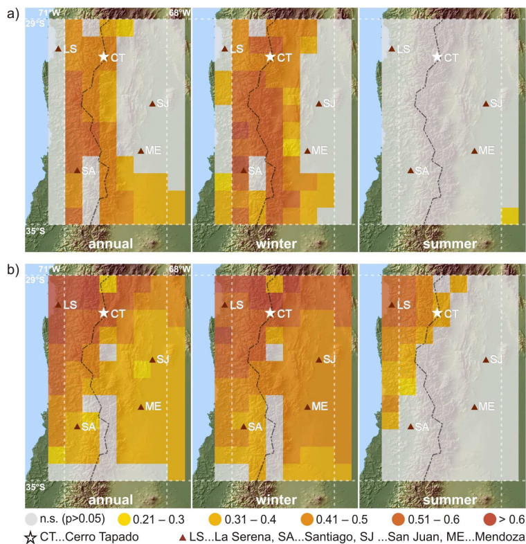
Fig. B2. Coefficients of the correlation analyses between annual as well as winter and summer (a) precipitation and (b) temperature after Willmott and Matsuura (2001) and the Niño 3.4 index of Trenberth and Stepaniak (2001) for the time period 1950 to 1999.
