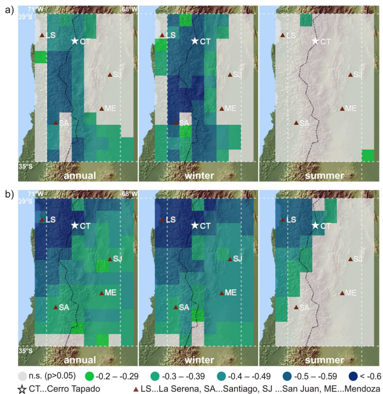
Fig. B1. Coefficients of the correlation analyses between annual as well as winter and summer (a) precipitation and (b) temperature after Willmott and Matsuura (2001) and the SOI of Allan et al. (1991) for the time period 1950 to 1999.
