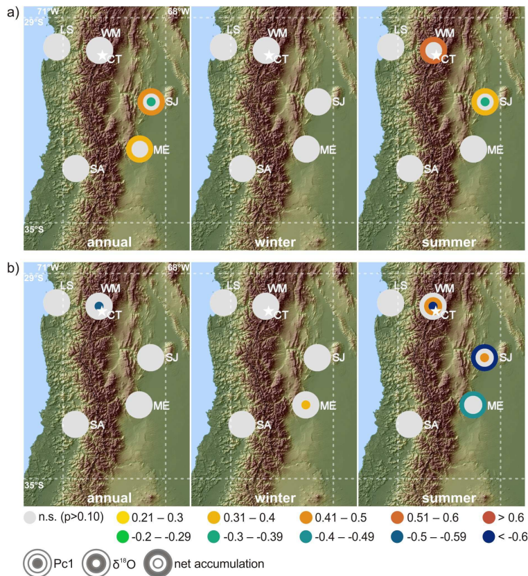
Fig. 8. Coefficients of correlation analyses between Tapado ice core proxies (inner to outer ring: PC1 of the major ion concentrations, \delta^{18}\text{O} and net accumulation) and meteorological data of (a) precipitation and (b) temperature. WM: glacier grids after Willmott and Matsuura (2001, see text), other abbreviations as in Fig. 4.
