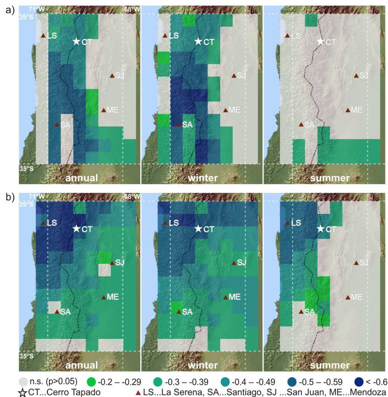
Fig. 4. Coefficients of the correlation analyses between annual as well as winter and summer (a) precipitation and (b) temperature time series after Willmott and Matsuura (2001) and the CEI of Gergis and Fowler (2005) for the time period 1950 to 1999.
