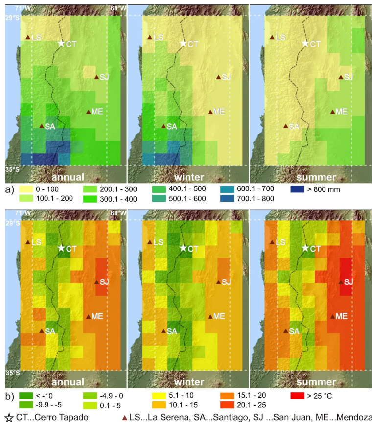
Fig. 3. Mean regional annual as well as winter and summer (a) precipitation amounts (mm) and (b) averaged temperatures (°C) in the subtropical Andes. Data after Willmott and Matsuura (2001) for the time period 1950 to 1999.
