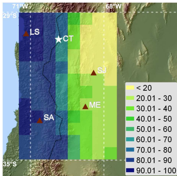
Fig. 7. Percentage winter precipitation of total annual precipitation in the subtropical Andes indicate the boundary between Mediterranean climate at the western and summer rain climate at the eastern Andean slopes (data: Willmott and Matsuura, 2001). Abbreviations as in Fig. 4.
