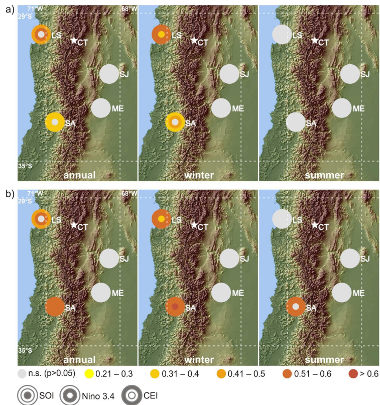
Fig. 6. Coefficients of three-year averaged correlation analyses between all ENSO indices (inner to outer ring: SOI, Niño 3.4 index and CEI) and meteorological station data of (a) precipitation and (b) temperature. Results are inverted for SOI and CEI. Abbreviations as in Fig. 4.
