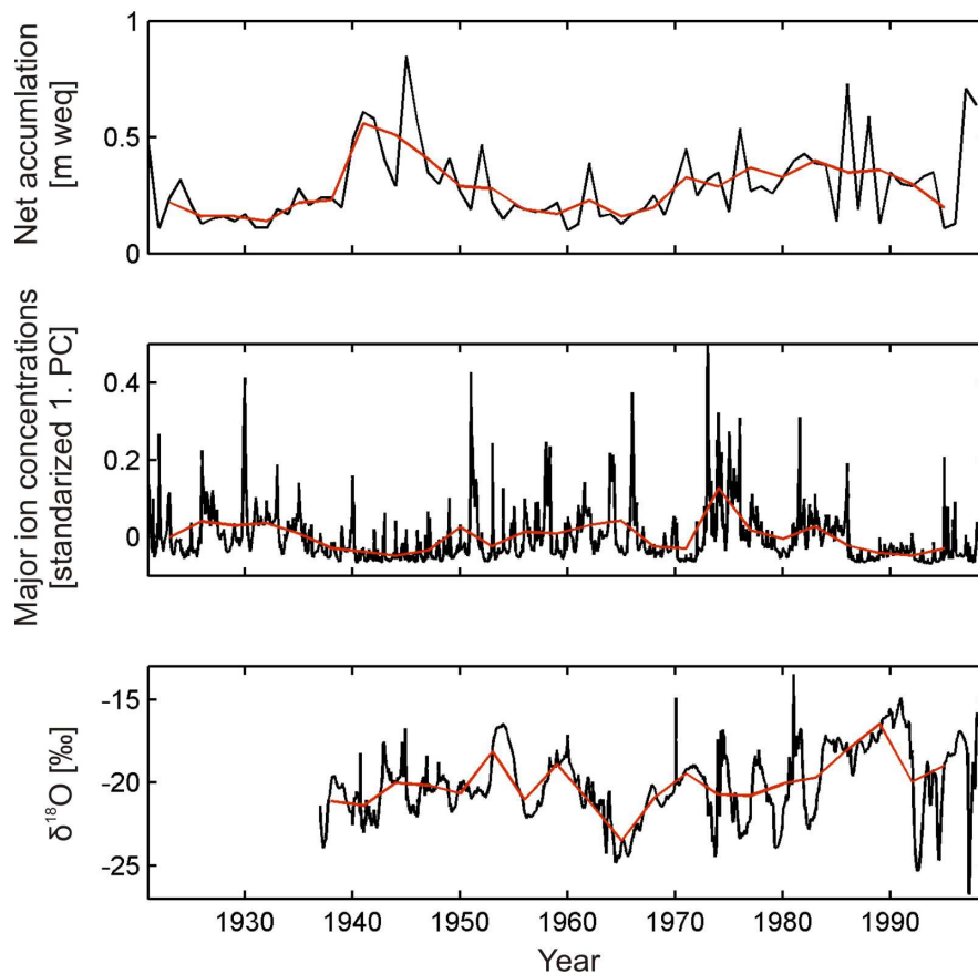
Fig. 2. Records of Cerro Tapado ice core proxies net accumulation, first PC of major ion concentrations and the \delta^{18}\text{O} -record (from top to bottom). Original data sets in black and three-year non-moving averages ending 1995 in red.
