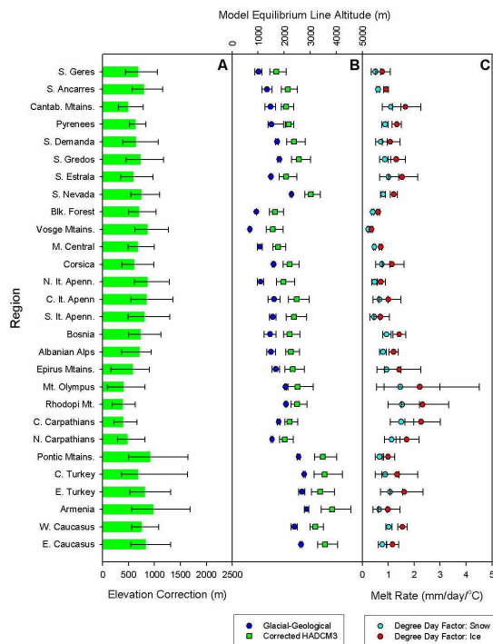
Fig. 9. Optimised elevation (Graph A) (with the adjusted ELA (Graph B)) and adjusted degree day factors melt factors (Graph C) required for the HadCM3 LGM climate anomalies to simulate equilibrium surface mass balance over the LGM glacier profiles of Europe and Eastern Black Sea reconstructed from glacial-geological evidence (Ehlers and Gibbard, 2004). The ELA reconstructions of Allen et al. (2007b) have are included in Graph B for comparison purposes. Locations of the glaciated regions are shown in Fig. 2. The range in results for each region (represented by minimum and maximum error bars) is caused by the suite of lapse rate combinations used to downscale the input climate onto the model glacier surface simulating different annual mass balance profiles and therefore different glaciological results.
