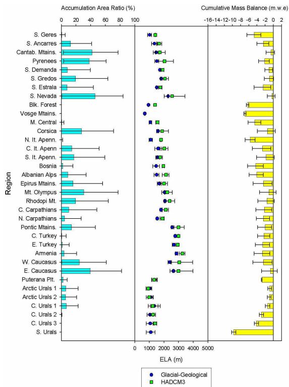
Fig. 8. HadCM3 21 k climate predictions of AAR, ELA, and cumulative mass balance for regions glaciated during the LGM (the location of regions can be found in Fig. 2). ELA predictions are plotted alongside the ELA estimates from Allen et al. (2007b) (labelled as glacial-geological). The range in results for each region (represented by minimum and maximum error bars) is caused by the suite of lapse rate combinations used to downscale the input climate onto the model glacier surface simulating different annual mass balance profiles and therefore different glaciological results.
