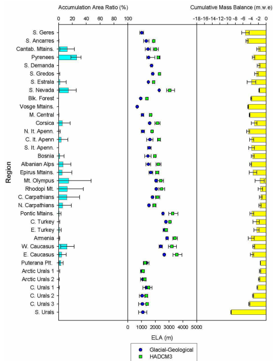
Fig. 4. HadCM3 LGM climate anomaly predictions of AAR, ELA, and cumulative mass balance for regions glaciated during the LGM (the location of regions can be found in Fig. 2). The AAR and cumulative mass balance results are calculated assuming that the fixed dimensions of the INQUA LGM glacier reconstructions (Ehlers and Gibbard, 2004) are correct. ELA predictions are plotted alongside the ELA estimates from the Allen et al. (2007b) (labelled as glacial-geological). The range in results for each region (represented by minimum and maximum error bars) is caused by the suite of lapse rate combinations used to downscale the input climate onto the model glacier surface simulating different annual mass balance profiles and therefore different glaciological results.
