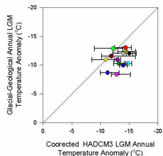
Fig. 6. Comparisons of “corrected” HadCM3 and glacial-geological LGM temperature anomalies from Allen et al. (2007b). The “correction” factor is shown in the left hand graph and the colour of these bars can be used to identify the temperature anomalies in the right hand graphs. The location of each region can be found in Fig. 2. The range of results (indicated by the minimum and maximum error bars) represents the variability in model climate caused by the use of a suite of lapse rates to downscale the climate onto the glacier surface (this is explained in Allen et al., 2007a). Note the axes on the temperature anomaly graphs have been inverted, the diagonal line is the 1:1 line; any data point plotting above the 1:1 line indicates the glacial-geological temperature anomaly is larger than the HadCM3 temperature anomaly for that region and vice versa for data points plotting below the 1:1 line.
