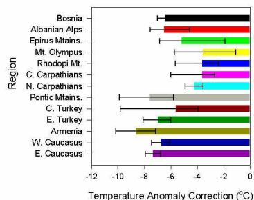
Fig. 6. Comparisons of “corrected” HadCM3 and glacial-geological LGM temperature anomalies from Allen et al. (2007b). The “correction” factor is shown in the left hand graph and the colour of these bars can be used to identify the temperature anomalies in the right hand graphs. The location of each region can be found in Fig. 2. The range of results (indicated by the minimum and maximum error bars) represents the variability in model climate caused by the use of a suite of lapse rates to downscale the climate onto the glacier surface (this is explained in Allen et al., 2007a). Note the axes on the temperature anomaly graphs have been inverted, the diagonal line is the 1:1 line; any data point plotting above the 1:1 line indicates the glacial-geological temperature anomaly is larger than the HadCM3 temperature anomaly for that region and vice versa for data points plotting below the 1:1 line.
