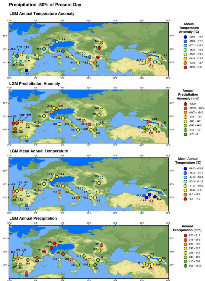
Fig. 6. Reconstructed LGM climates across Europe and Black Sea simulated using -80\% of present day annual precipitation totals derived from the CRU2.0 climate dataset (New et al., 2002). Reconstructions of LGM glaciers are adapted from the INQUA database (Ehlers and Gibbard, 2004a).
