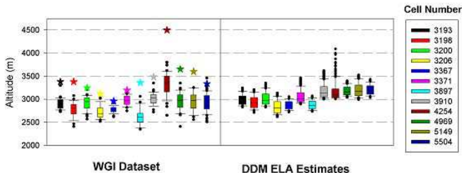
Fig. 6. WGI (National Snow and Ice Data Center, 1999) within cell altitude distributions and DDM ELA estimates in the Alps. The maximum glacierised altitude in the WGI dataset is indicated by the star, the boxplot beneath the star is the altitudinal distribution of WGI snowline measurements within the cell. For identification purposes during model simulations cells in the ~20 km resolution model domains (see Table 3) were numbered starting from the top left hand corner of the model grid and finished at the bottom right hand corner, each row was numbered left to right. Cell numbers have been included in this diagram to help the reader compare WGI data (left hand panel) and DDM results (right hand panel) from the same cell.
