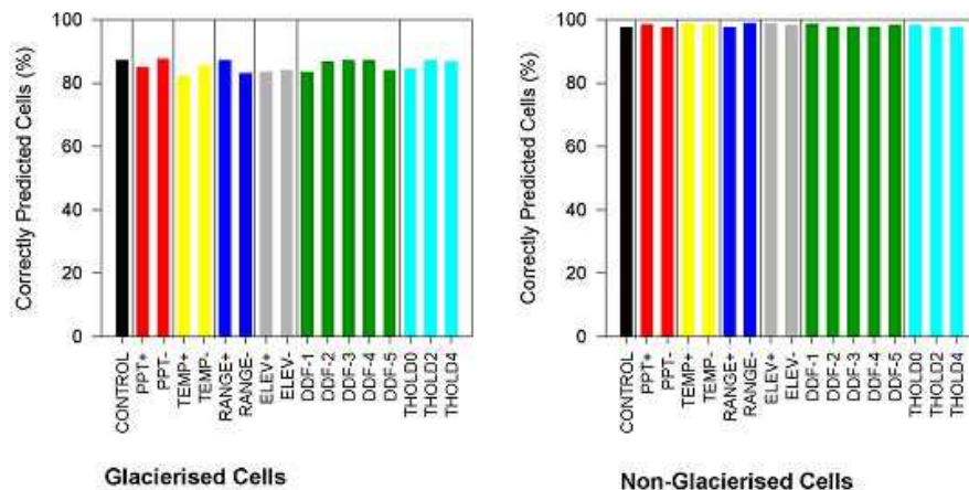
Fig. 7. Percentage of correctly predicted glacierised and non-glacierised cells across the suite of sensitivity analyses for the Alps. See Table 6 for details of individual sensitivity experiments.
