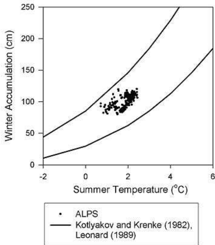
Fig. 5. Climate at the ELA predicted by the DDM in the Alps using the optimum lapse rate combinations derived in Experiment One compared to ELA climates measured on present day mid-latitude mountain glaciers (Kotlyakov and Krenke, 1982; Leonard, 1989).
