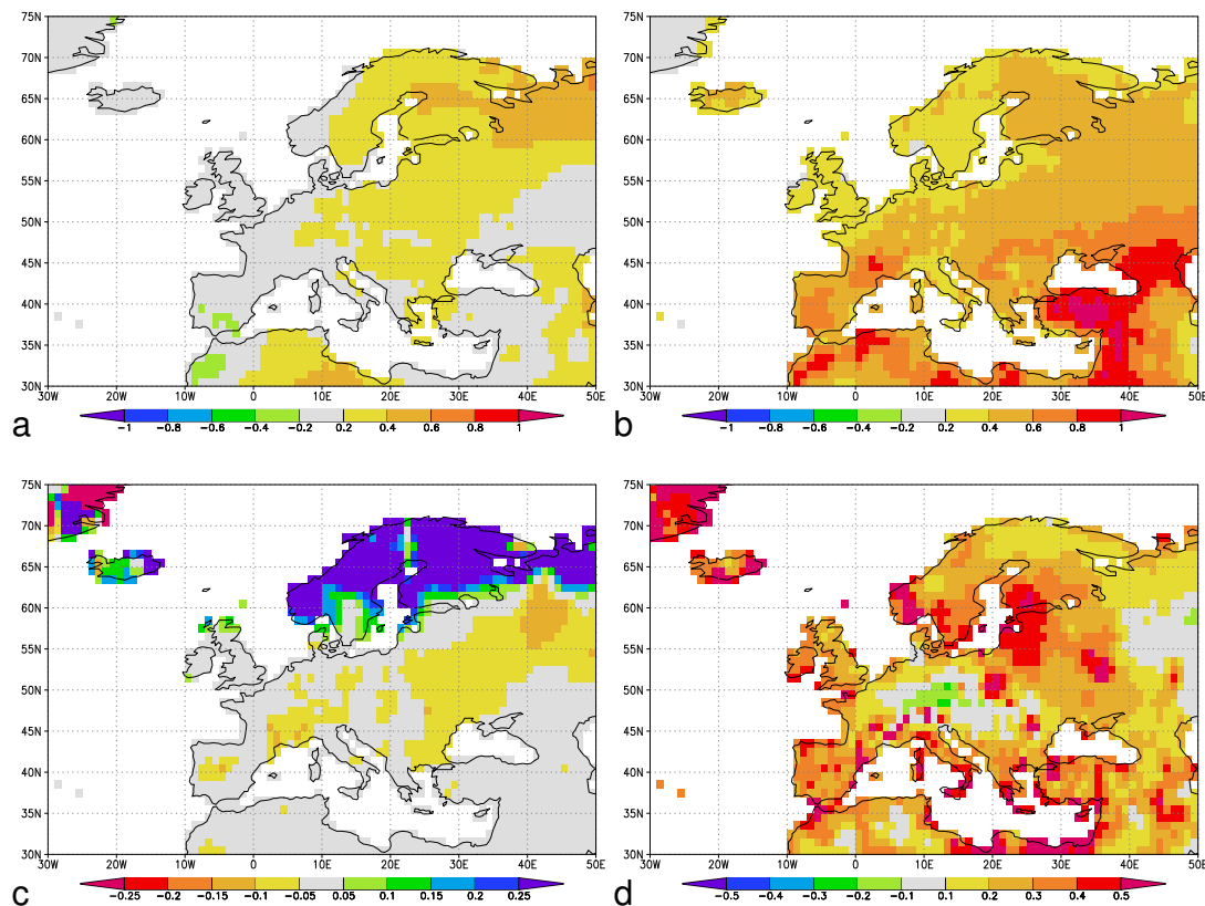
Fig. 9. The coefficients of the VSM Eqs. (2–4) averaged over September–November: zonal geostrophic wind A_W [ \text{Km}^{-1}\text{s} ] (a), the meridional zonal wind A_S [ \text{Km}^{-1}\text{s} ] (b), the solar radiation B [ \text{KW}^{-1}\text{m}^2 ] (c); the memory term M in September (d).
