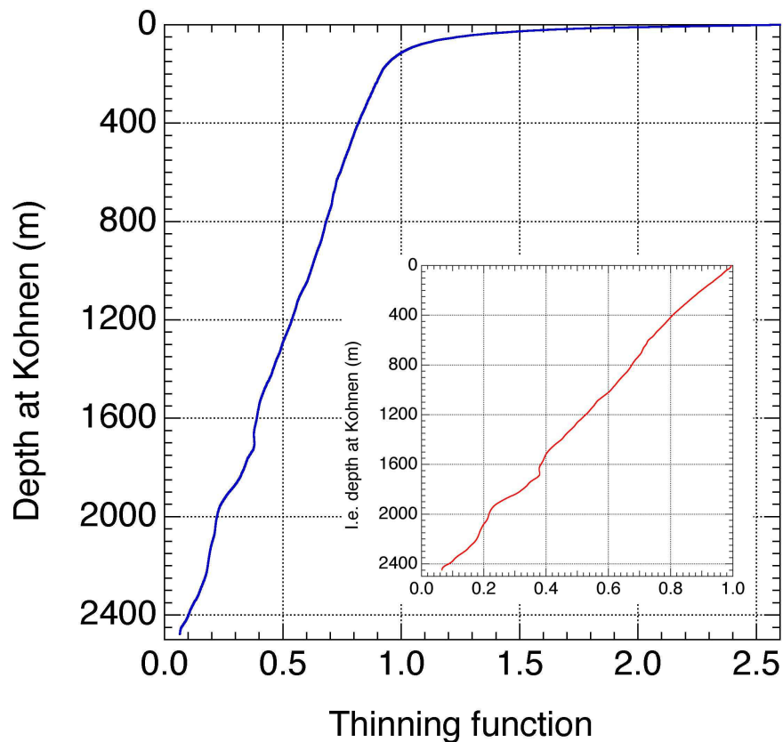
Fig. 12. Thinning function at Kohnen plotted as a function of depth. The blue line is plotted versus real depth and was corrected for a variable firn density in the upper 180m. The inset shows the original thinning function obtained in the experiment as a function of ice equivalent depth.
