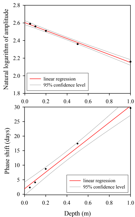
Fig. 12. Natural logarithm of amplitude (upper panel) and phase shift relative to the SAT (bottom panel) as function of depth for Bistrița. The coefficient of determination of the regression line is r^2=0.996 and r^2=0.990 for amplitude and phase shift, respectively. The 95% confidence interval is also included.
