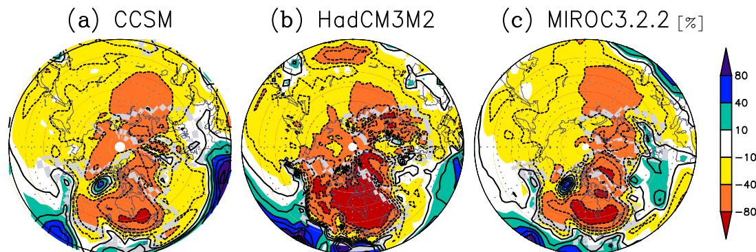
Fig. 5. Ratio of annual precipitation change in per cent for PMIP2 models: (a) CCSM, (b) HadCM3M2, (c) MIROC3.2.2 by using (LGM – CTL)/CTL. The contour interval is 20 %.
