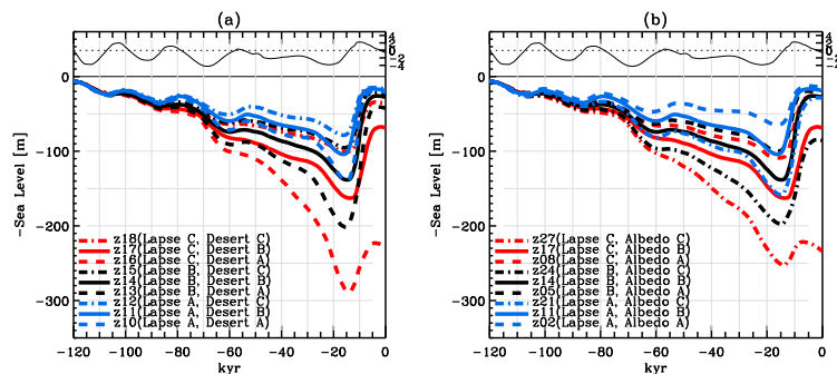
Fig. 8. Same as Fig. 7 but for the past 120 000 years and different cases depending on lapse rate, albedo-effect and desertification rate parameter. Lapse A = 4.0 \text{ K km}^{-1} , Lapse B = 5.0 \text{ K km}^{-1} , Lapse C = 6.0 \text{ K km}^{-1} ; Desert A = 0.01 , Desert B = 0.022 , Desert C = 0.04 ; Albedo A = -3.7 \times 10^{-13} \text{ K m}^{-2} , Albedo B = -4.7 \times 10^{-13} \text{ K m}^{-2} , Albedo C = -5.7 \times 10^{-13} \text{ K m}^{-2} . The lapse rate parameter corresponds to \lambda in Eq. (9). The desertification rate parameter corresponds to d_0 in Eq. (11). Albedo effect parameter corresponds to \gamma_{\text{area}} in Eq. (10).
