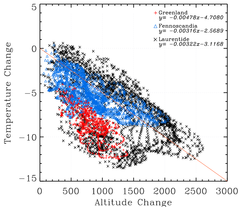
Fig. 2. Difference in summer surface temperature (mean of June, July and August) versus the difference in altitude for all the grid points over the ice sheet in the model. The red line corresponds to the relation of the lapse rate -5^{\circ}\text{C per km} . The red mark of scatter plots is for Greenland ice sheet, the blue mark for Fennoscandian ice sheet, and the black mark is for Laurentide ice sheet.
