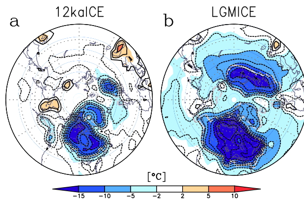
Fig. 3. Same as Fig. 1c, but for different sizes of “flat” ice sheet (at LGM and 12 ka). (a) M12flat–M21nice, (b) M21flat–M21nice.
