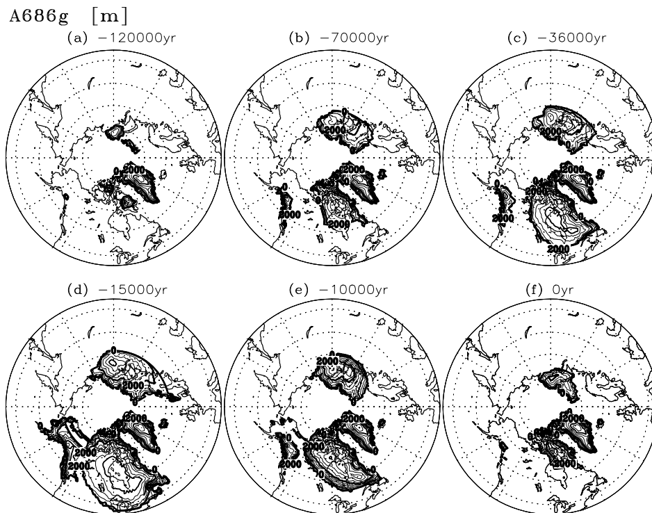
Fig. 7. Ice sheet distribution at different stages at (a) 120 ka, (b) 70 ka, (c) 36 ka, (d) 15 ka, (e) 10 ka, (f) 0 ka. Contour intervals are 250 m (thin), 1000 m (thick) and 2000 m (labeled). The volume of each ice sheet in terms of sea level contribution is (a) -6.278 m, (b) -51.643 m, (c) -90.253 m, (d) -137.827 m, (e) -77.167 m, (f) -27.095 m.
