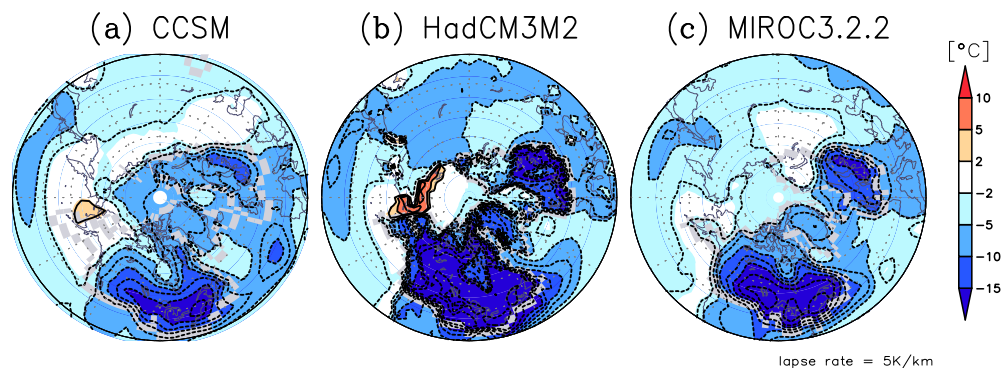
Fig. 4. Same as Fig. 1 but for PMIP2 models. (a) CCSM, (b) HadCM3M2, (c) MIROC3.2.2. Change in summer surface air temperature but the lapse rate effect ( = 5 \text{ K km}^{-1} for each modelled ice sheet topography) is extracted.
