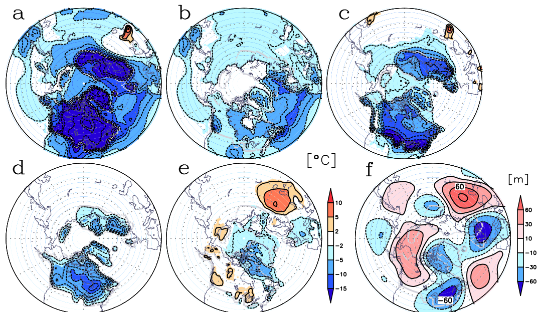
Fig. 1. Difference in summer surface air temperature (mean of June, July and August) in °C due to boundary conditions for (a) to (e) , and difference in summer geopotential height at 500 hPa level for (f) . (a) Total difference by experiments (LGMfull–CTLH), (b) CO 2 and SST effect by experiments (LGMnice–CTLH), (c) Albedo effect by experiments (LGMflat–LGMnice), (d) Topography Lapse Rate Effect assuming a lapse rate 5 K km -1 for the given topography (LGMfull–LGMflat), (e) Topography effect other than the lapse rate effect as Residual (e=a–b–c–d). (f) Difference in summer geopotential height at 500 hPa level due to ice sheet topography (LGMfull–LGMflat). Contours of Figs. (a) to (e) are at: –50, –45, –35, –30, –25, –20, –17.5, –15, –12.5, –10, –7.5, –5, –2.5, 2.5, 5, 7.5, 10, 12.5. Contours of Fig. (f) are at: –150, –120, –90, –60, –30, –10, 10, 30, 60, 90, 120, 150. Gray line in the figures indicates the ice sheet extent used in the GCM.
