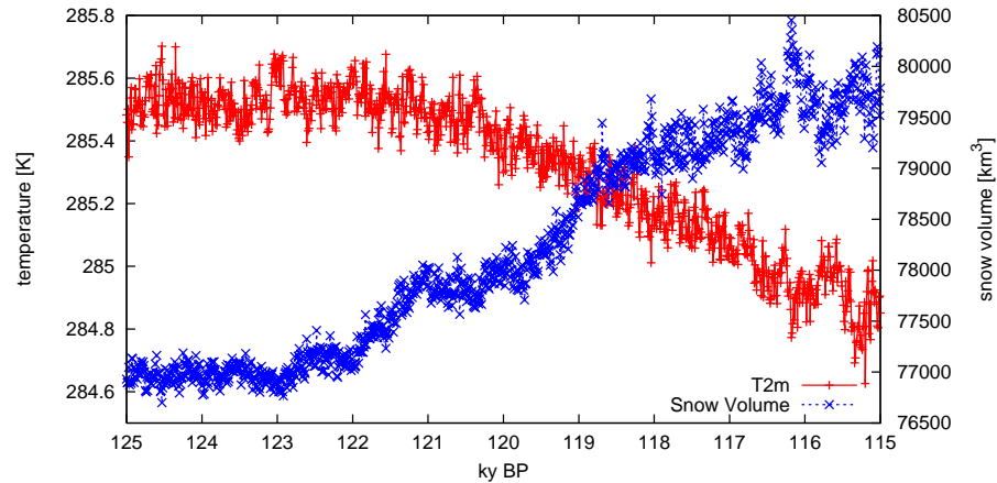
Fig. 6. Global snow volume in km 3 and annual global mean temperature in the transient simulation.
