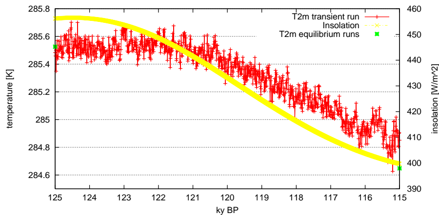
Fig. 5. Annual global mean temperature [K] of the transient simulation and of the equilibrium runs and solar insolation [W/m 2 ] during summer (JJA) at 65° N.
