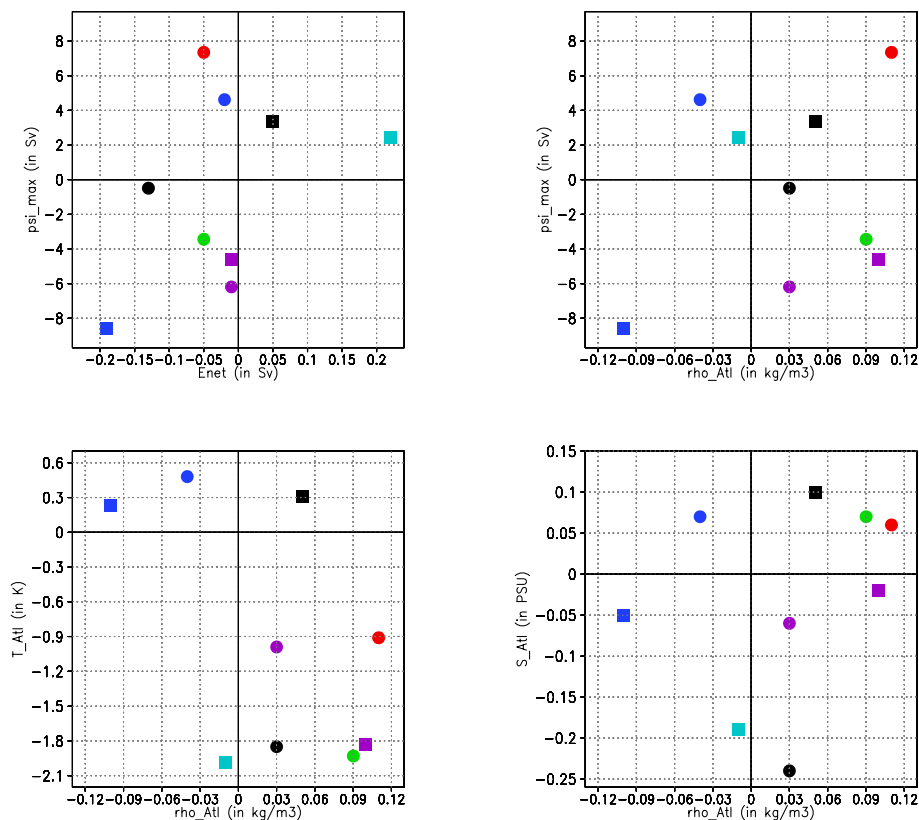
Fig. 4. The response in the maximum of the Atlantic THC strength versus that in net evaporation (upper left panel) and versus that in the north-south Atlantic density difference \rho_{\text{Atl}} (upper right panel) for the PMIP2 (circles) and PMIP1.5 (squares) simulations. Color coding as in Fig. 2. The lower panels give the response in the north-south Atlantic temperature difference and salinity difference versus \Delta\rho_{\text{Atl}} : negative values on the vertical axis indicate that the northern Atlantic cools and freshens during the LGM as compared to the southern part.
