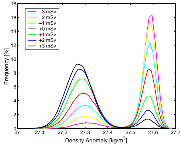
Fig. 10. Histograms (probability density functions) of Labrador Sea density-anomalies in the stochastically forced ( \sigma=0.2 Sv) conceptual model for different constant freshwater perturbations P' between -3 mSv and +3 mSv.
