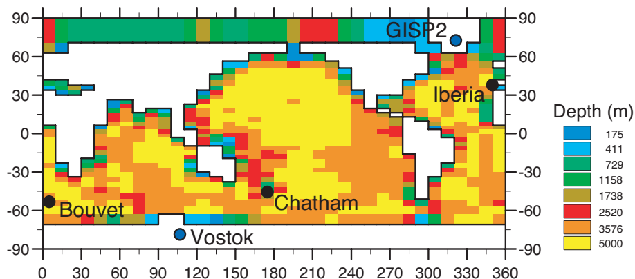
Fig. 1. Model ocean bathymetry on the GENIE-1 horizontal grid: 36 \times 36 cells in constant increments of longitude and \sin(\text{latitude}) . Also indicated are the three sediment core sites (Iberian Margin, Bouvet Island, Chatham Rise – black dots) and the two ice core stations (GISP2, Vostok – blue dots).
