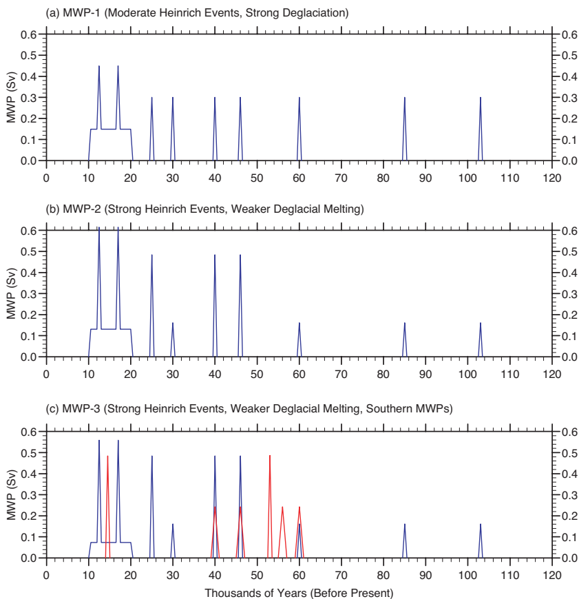
Fig. 5. Time series of Meltwater Pulses: (a) MWP-1; (b) MWP-2; (c) MWP-3 (see text for details). The colours identify where the MWPs are applied: blue, equally at ocean gridboxes in the Atlantic zone 50–70° N; red, equally at coastal ocean gridboxes around Antarctica.
