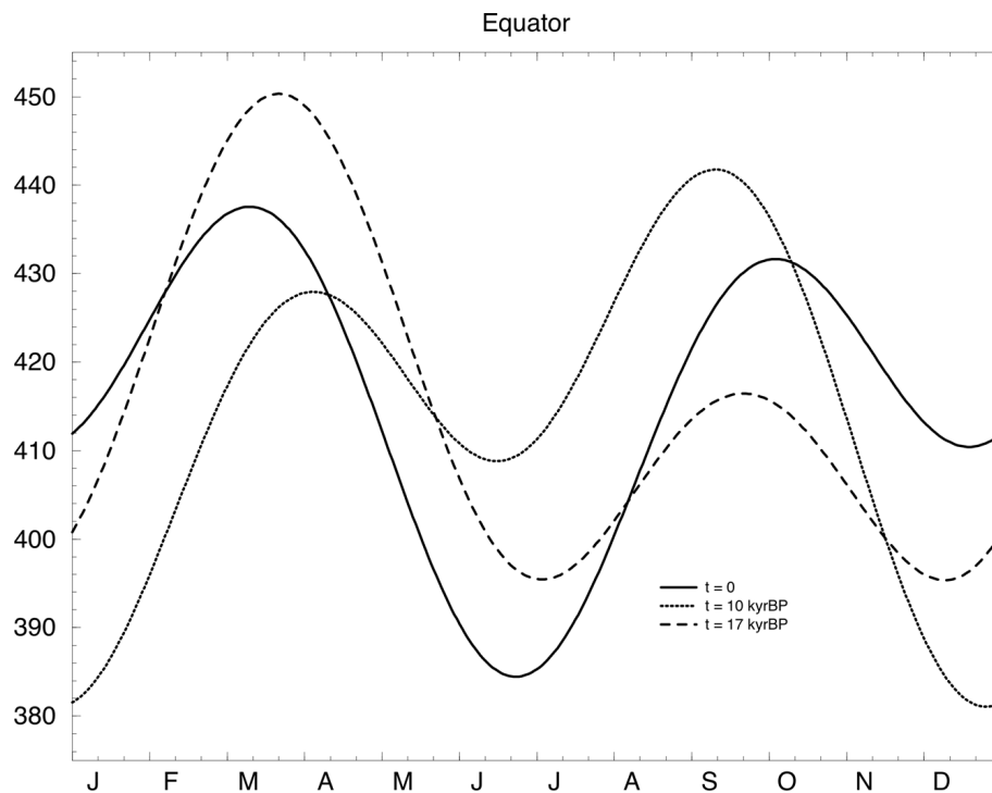
Fig. 1. Seasonal cycle of insolation at the equator at present (full line), at 10 kyr BP (dotted line) and at 17 kyr BP (dashed line). Units are \text{Wm}^{-2} .
