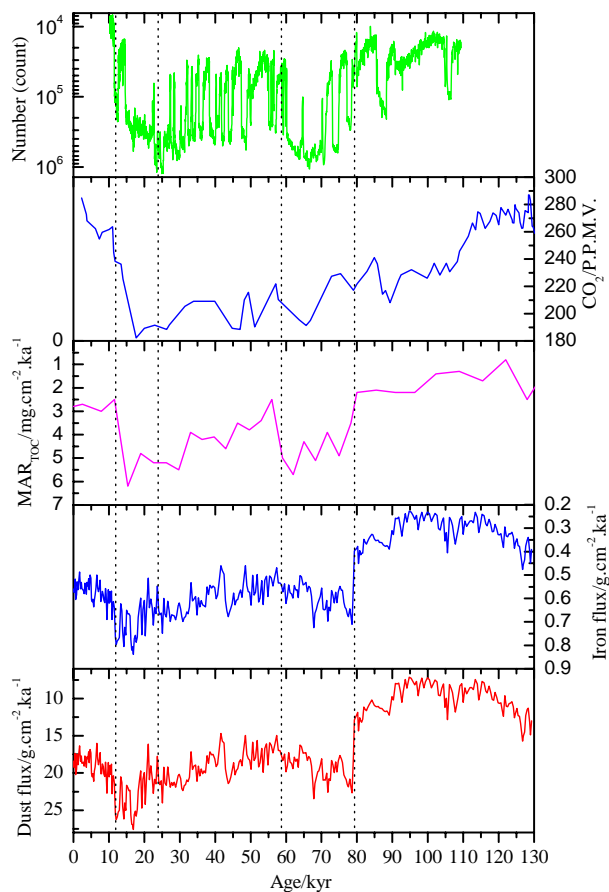
Fig. 4. Correlations between Asian dust and iron fluxes recorded in Lingtai loess profile, dust particulate counts of GRIP ice core, paleoproductivity represented in MAR_{TOC} variations of H3571 core of northern Pacific ocean, and atmospheric CO_2 recorded in Vostok ice core during the last 130 kyr.
