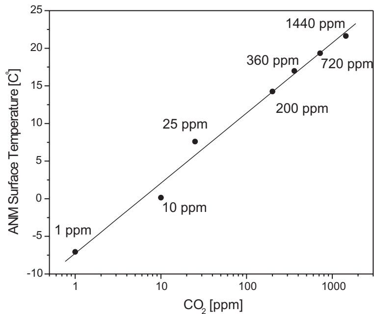
Fig. 5. Log plot of the carbon dioxide concentration versus ANM surface temperature for exp. Exp_1, Exp_10, Exp_25, Exp_200, Exp_360, Exp_720 and Exp_1440. The line shows the linear fit.
