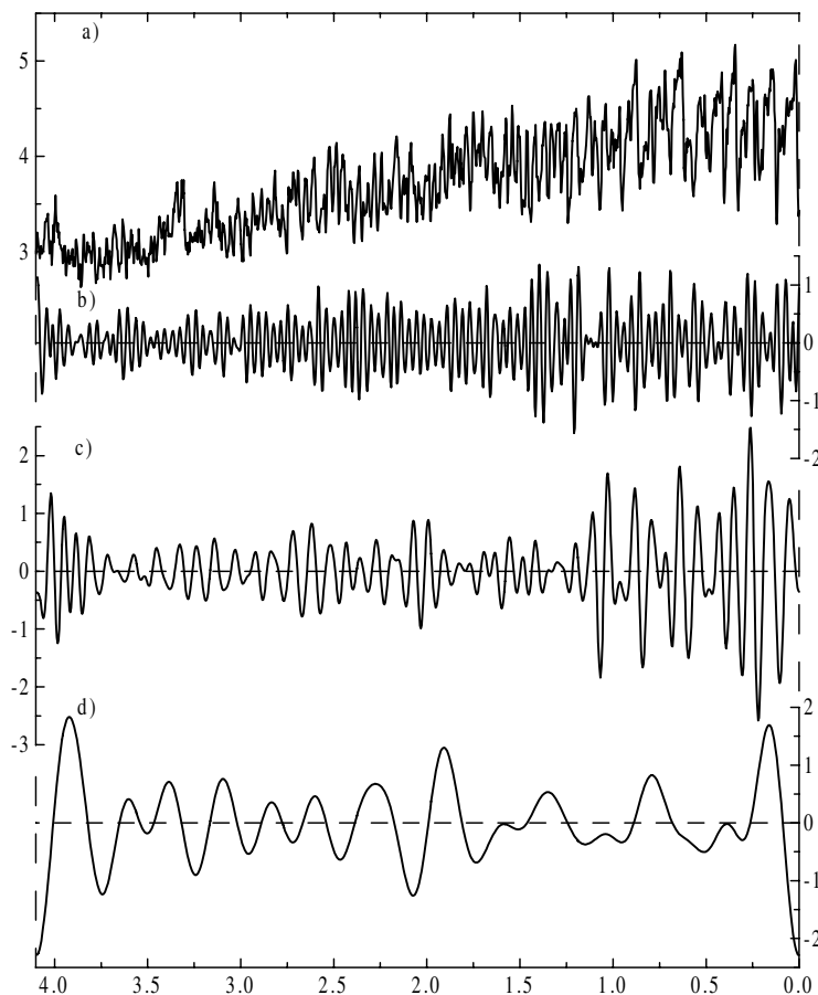
Fig. 4. (a) Time series of oxygen isotope ratios, \delta^{18}\text{O} , and detail components derived by the non-decimated wavelet transform – (b) D_8 , (c) D_7 , and (d) D_5 with the periods of \sim 40 , 100, and 400 ky, respectively. X-axis is the ky BP.
