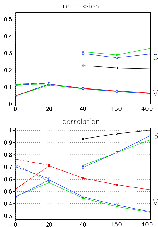
Fig. 2. (a) The regression (in °C per W/m 2 ) for different low-pass filter periods (in yr) of the NH temperatures on the volcanic and solar forcing, indicated by V and S, in the ECBilt experiments driven by solar-volcanic forcing (blue and green lines), solar forcing alone (black line) and volcanic forcing alone (red line), and (b) same for the correlation. The temperature data are smoothed with a 10-yr low-pass filter prior to the analysis (dotted lines give results for the unsmoothed data) for later comparison with the proxy-based estimates.
