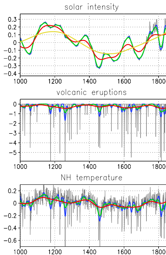
Fig. 1. The radiative forcing due to variations in solar intensity (upper panel), volcanic eruptions (middle panel; both in W/m^2 ) and the simulated anomalies in NH temperature (in ^{\circ}C ) from one of the volcanic-solar forced runs with the ECBilt climate model for the pre-anthropogenic period (time in years AD). Also shown are the smoothed records, using low-pass filter periods of 20 yr (blue), 40 yr (green), 150 yr (red) and 400 yr (yellow; solar forcing only).
