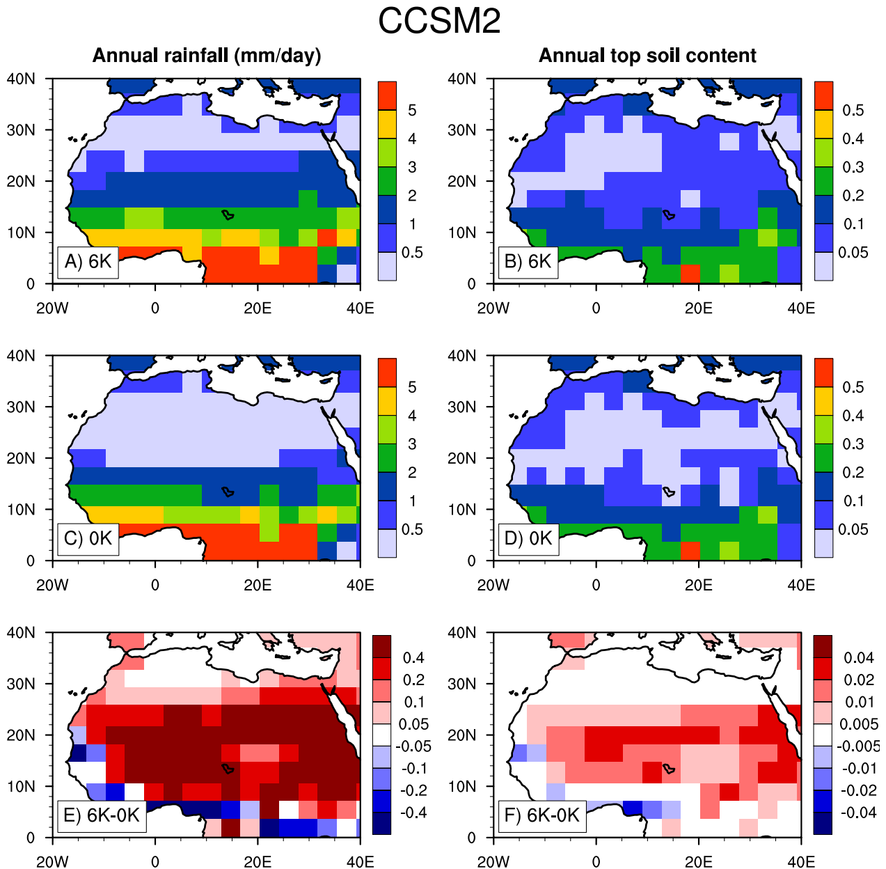
Fig. 3. Annual rainfall (mm/day) for CCSM2 (A) 6K control, (C) 0K control, and (E) 6K minus 0K. Top soil moisture content ( \text{mm}^3/\text{mm}^3 ) for CCSM2 (B) 6K control, (D) 0K control, and (F) 6K minus 0K from two sets of 350-year control simulations.
