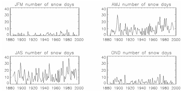
Fig. 2. Seasonal snowfall frequency (number of events).
