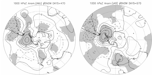
Fig. 4. Autumn (AMJ) and winter (JAS) 1000-hPa geopotential height anomalies (gpm) during snowfall days for the 1958–1996 period relative to the corresponding seasonal average for the same period at 10 gpm intervals. Positive/negative anomalies are displayed with continuous/dashed lines. 99% significant differences with respect to the seasonal geopotential height average are shaded. The total number of snowfall days in the sample is displayed above each graph.
