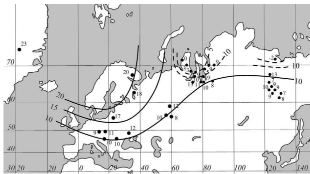
Fig. 2. The spatial distribution of the geothermal estimates of PHW amplitude in Northern Eurasia (K). Solid lines represent the main pattern the distribution follows; dashed lines show local anomalies.
