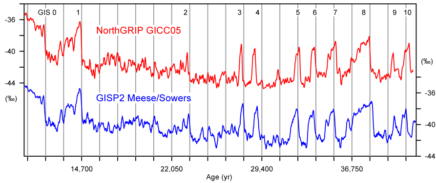
Fig. 1. The \delta^{18}\text{O} isotope records from NGRIP and GISP2 on their stratigraphic time scales (Alley et al., 1997; Andersen et al., 2006). The vertical bars are separated by 1470 years. The analysis focus on the well defined fast onsets of DO events, which are the transitions from the stadial to the interstadial states. Beginning at GIS0 the onset for the DO events are for the NGRIP GICC05 (GISP2) time scale: 11 700 (11 660); 13 130 (13 180); 14 680 (14 700); 23 340 (23 560); 27 780 (27 920); 28 900 (29 100); 32 500 (32 400); 33 740 (33 700); 35 480 (35 360); 38 220 (38 480); 40 160 (40 280); 41 460 (41 240). Ages are b2k=BP+50 years.
