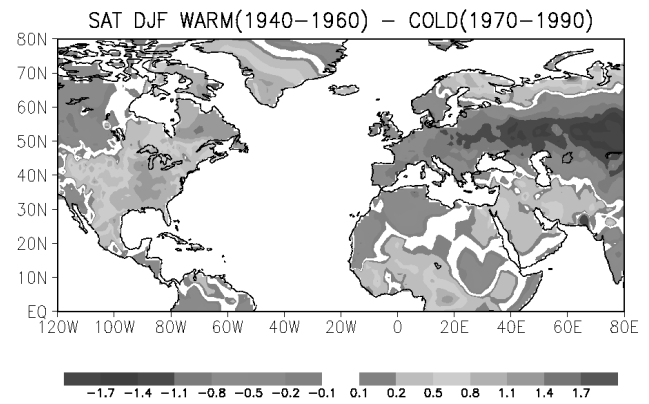
Fig. 5. Anomalous warm – cold SAT (same as for Figs. 4b, c, d) over land, derived from CRU-TS2.1 monthly climate observations (Mitchell and Jones, 2005).
