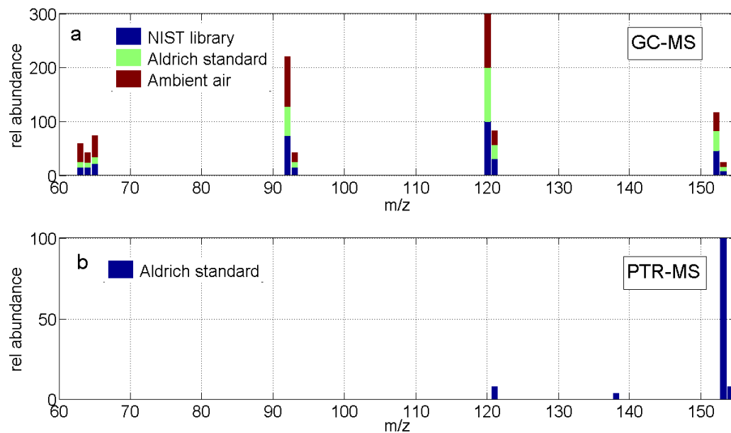
Fig. 1. (a). Stacked bar plot of electron-impact ionization mass spectra of methyl salicylate (NIST library, an authentic standard (SigmaUltra, Sigma Aldrich, CAS 119-36-8, Milwaukee, WI) and ambient air measurements). (b). Proton-transfer-reaction mass spectra of methyl salicylate using an authentic standard (SigmaUltra, Sigma Aldrich, CAS 119-36-8, Milwaukee, WI).
