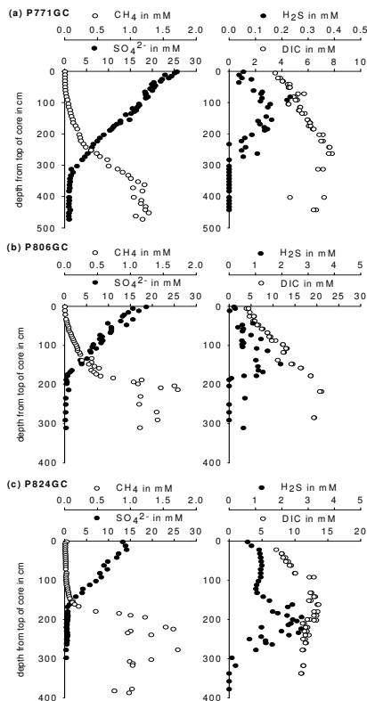
Fig. 2. Pore water concentration profiles of \text{CH}_4 , \text{SO}_4^{2-} , \text{H}_2\text{S} and DIC in gravity cores from the three stations. The top of the core is not identical with the sediment surface because some sediment might have been lost by coring.
