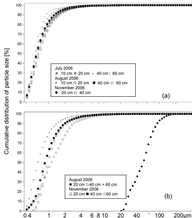
Fig. 2. Sum curves [cumulative %] of particle size in the POM fraction (>0.45 μm) at different managed peatlands of the Donauried (Germany), (a) re-wetted fen, (b) moderately drained fen at distinct sampling depths and times.
