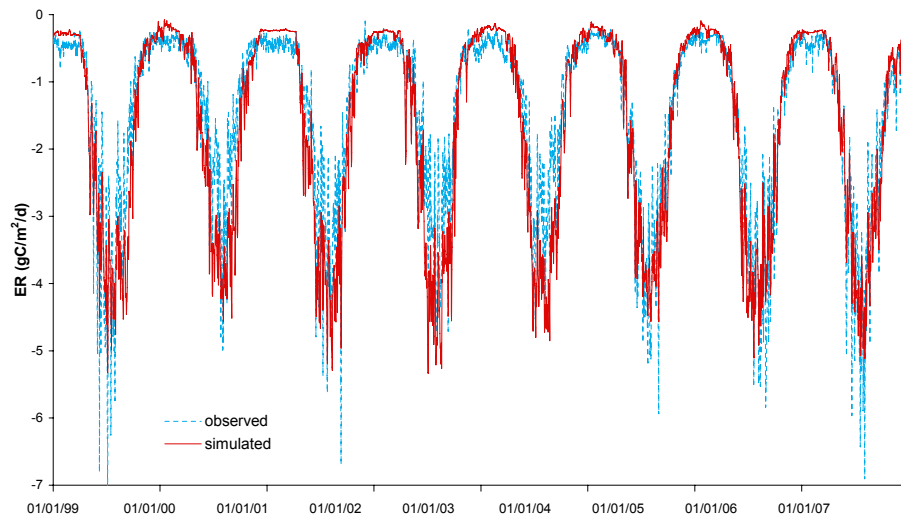
Fig. 3. The time series of hourly measured (blue dashed line) and simulated (red solid line) ER for 1999–2006.
