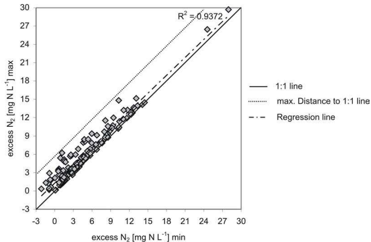
Fig. 2. Minimum and maximum estimates of excess N 2 for the whole data set as calculated using Eqs. (1) and (2) or (1) and (3), respectively.
